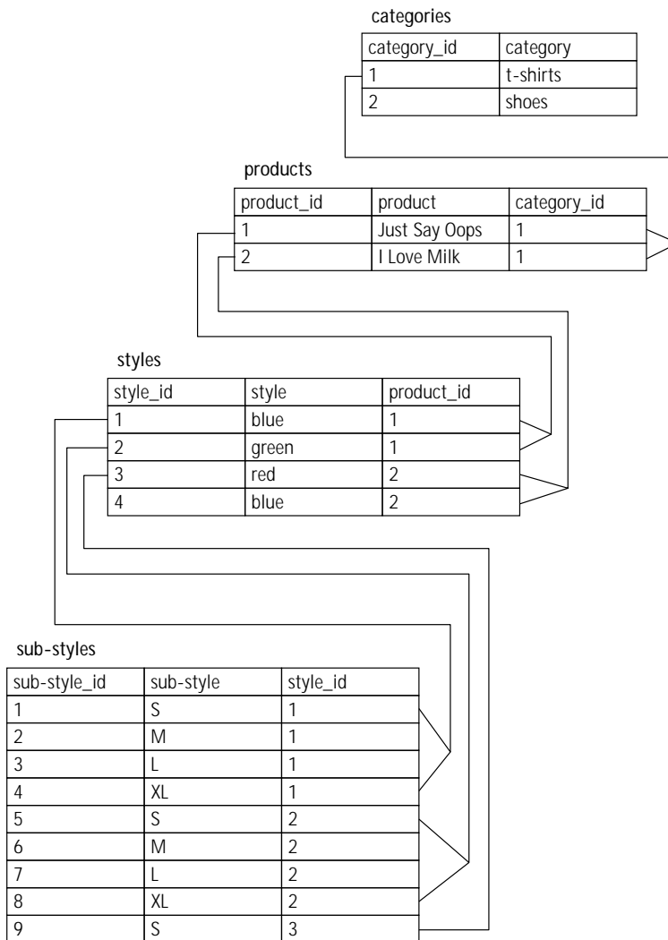
Figure 10-8: Sample hierarchical data
