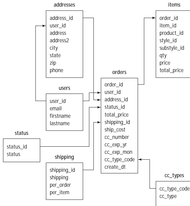
Figure 14-5: Cart schema
