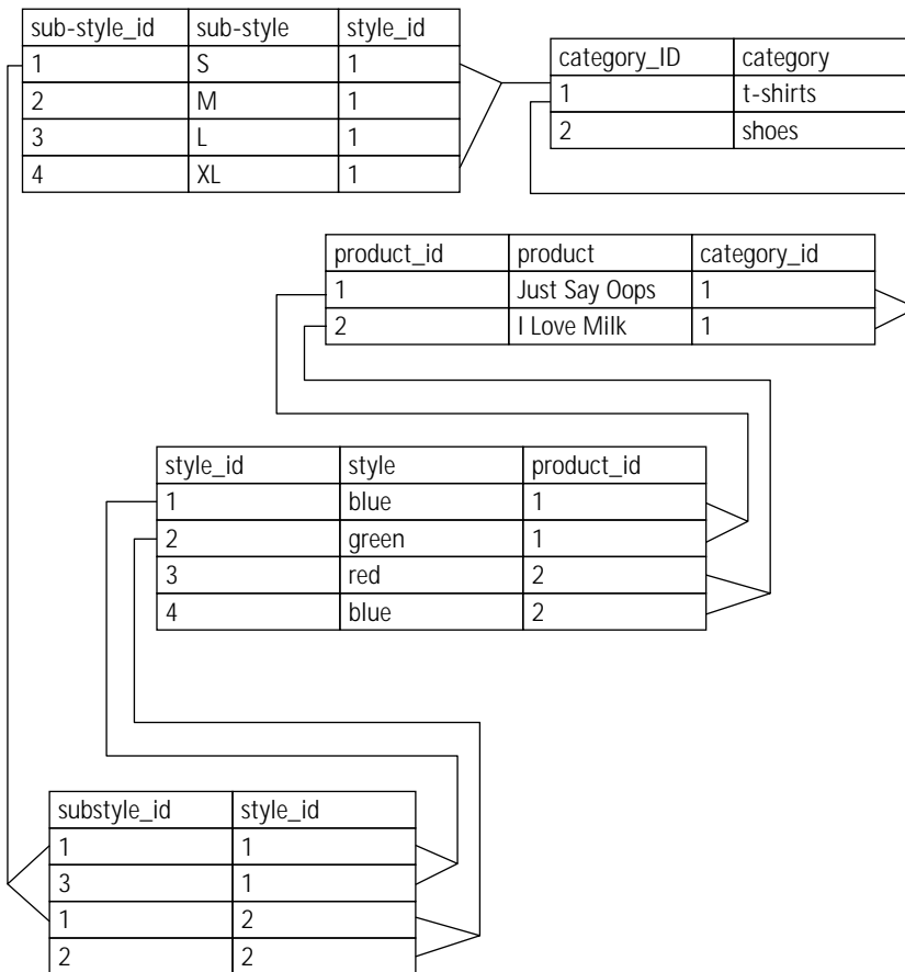
Figure 10-10: Sample data
