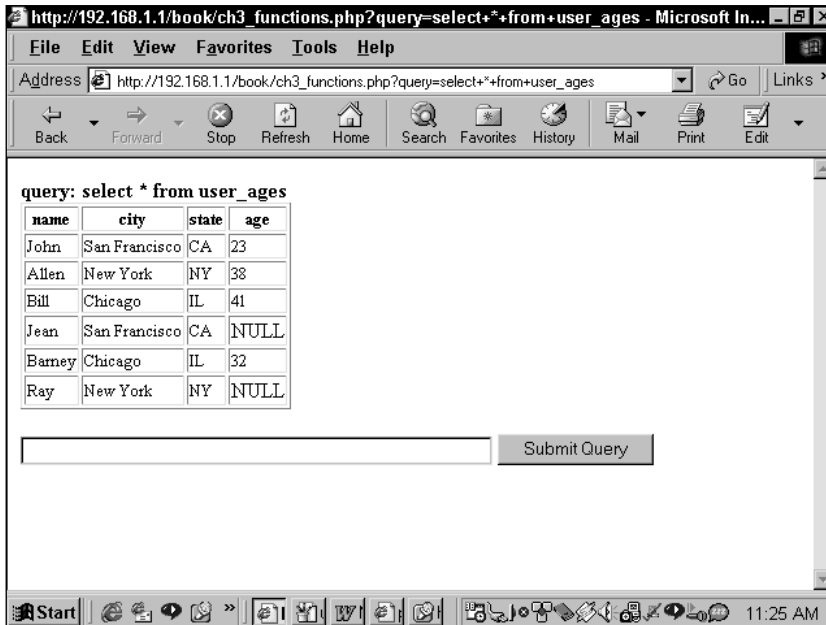
Figure 3-6: users_ages table
