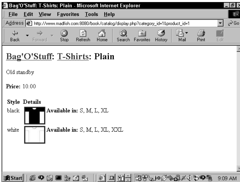
Figure 10-3: Items list
