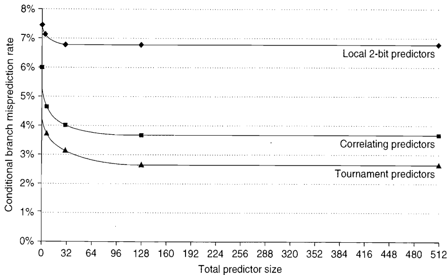
Figure 3.4 The misprediction rate for three different predictors on SPEC89 as the total number of bits is increased. The predictors are a local 2-bit predictor, a correlating predictor that is optimally structured in its use of global and local information at each point in the graph, and a tournament predictor. Although these data are for an older version of SPEC, data for more recent SPEC benchmarks would show similar behavior, perhaps converging to the asymptotic limit at slightly larger predictor sizes.
