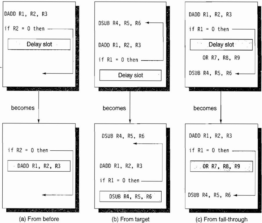
Figure C.14 Scheduling the branch delay slot. The top box in each pair shows the code before scheduling; the bottom box shows the scheduled code. In (a), the delay slot is scheduled with an independent instruction from before the branch. This is the best choice. Strategies (b) and (c) are used when (a) is not possible. In the code sequences for (b) and (c), the use of R1 in the branch condition prevents the DADD instruction (whose destination is R1) from being moved after the branch. In (b), the branch delay slot is scheduled from the target of the branch; usually the target instruction will need to be copied because it can be reached by another path. Strategy (b) is preferred when the branch is taken with high probability, such as a loop branch. Finally, the branch may be scheduled from the not-taken fall-through as in (c). To make this optimization legal for (b) or (c), it must be OK to execute the moved instruction when the branch goes in the unexpected direction. By OK we mean that the work is wasted, but the program will still execute correctly. This is the case, for example, in (c) if R7 were an unused temporary register when the branch goes in the unexpected direction.
