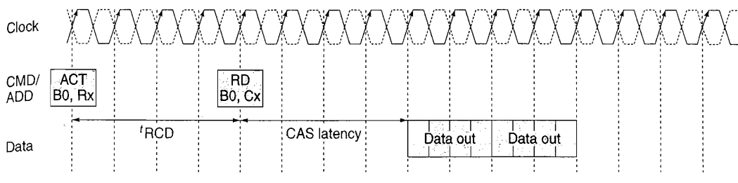
Figure 2.31 DDR2 SDRAM timing diagram.
