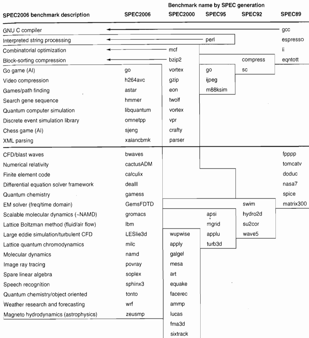
Figure 1.16 SPEC2006 programs and the evolution of the SPEC benchmarks over time, with integer programs above the line and floating-point programs below the line. Of the 12 SPEC2006 integer programs, 9 are written in C, and the rest in C++. For the floating-point programs, the split is 6 in Fortran, 4 in C++, 3 in C, and 4 in mixed C and Fortran. The figure shows all 70 of the programs in the 1989, 1992, 1995, 2000, and 2006 releases. The benchmark descriptions on the left are for SPEC2006 only and do not apply to earlier versions. Programs in the same row from different generations of SPEC are generally not related; for example, fpppp is not a CFD code like bwaves. Gcc is the senior citizen of the group. Only 3 integer programs and 3 floating-point programs survived three or more generations. Note that all the floating-point programs are new for SPEC2006. Although a few are carried over from generation to generation, the version of the program changes and either the input or the size of the benchmark is often changed to increase its running time and to avoid perturbation in measurement or domination of the execution time by some factor other than CPU time.
