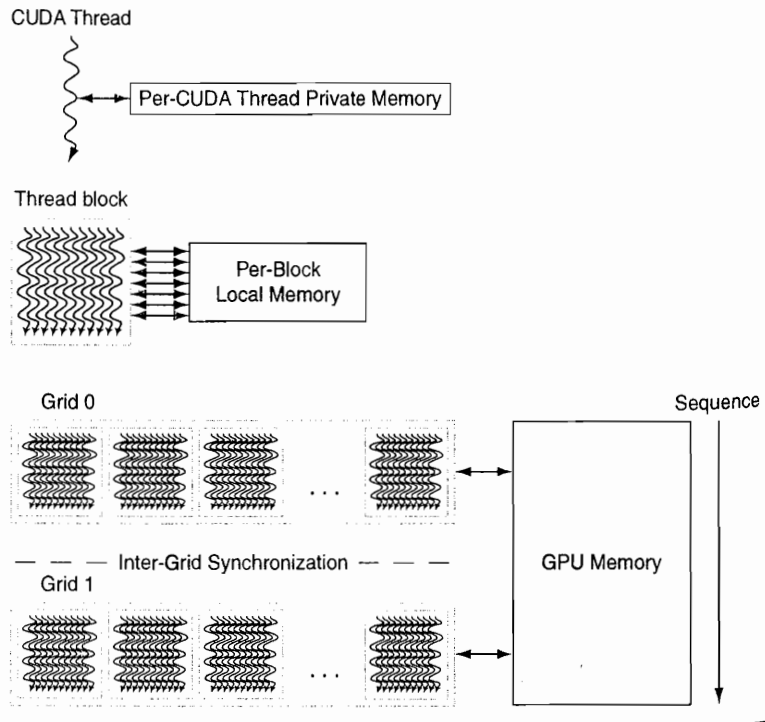
Figure 4.18 GPU Memory structures. GPU Memory is shared by all Grids (vectorized loops), Local Memory is shared by all threads of SIMD instructions within a thread block (body of a vectorized loop), and Private Memory is private to a single CUDA Thread.
