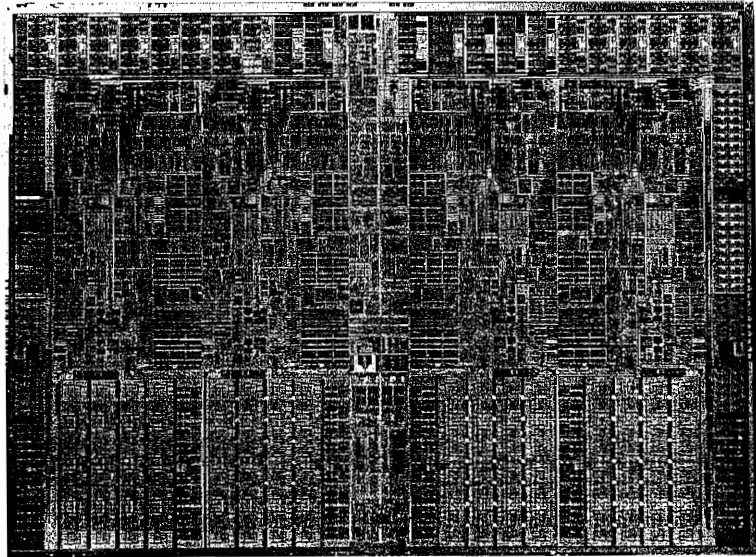
Figure 1.13 Photograph of an Intel Core i7 microprocessor die, which is evaluated in Chapters 2 through 5. The dimensions are 18.9 mm by 13.6 mm (257 mm 2 ) in a 45 nm process. (Courtesy Intel.)
