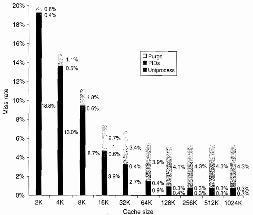
Figure B.16 Miss rate versus virtually addressed cache size of a program measured three ways: without process switches (uniproccess), with process switches using a process-identifier tag (PID), and with process switches but without PIDs (purge). PIDs increase the uniproccess absolute miss rate by 0.3% to 0.6% and save 0.6% to 4.3% over purging. Agarwal [1987] collected these statistics for the Ultrix operating system running on a VAX, assuming direct-mapped caches with a block size of 16 bytes. Note that the miss rate goes up from 128K to 256K. Such nonintuitive behavior can occur in caches because changing size changes the mapping of memory blocks onto cache blocks, which can change the conflict miss rate.
