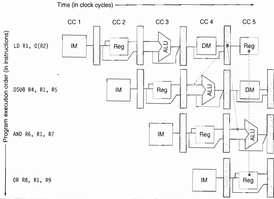
Figure C.9 The load instruction can bypass its results to the AND and OR instructions, but not to the DSUB, since that would mean forwarding the result in “negative time.”
