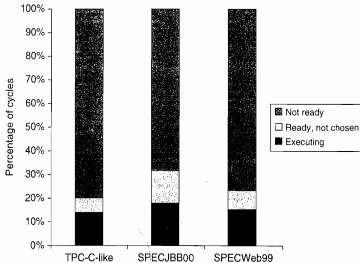
Figure 3.31 Breakdown of the status on an average thread. “Executing” indicates the thread issues an instruction in that cycle. “Ready but not chosen” means it could issue but another thread has been chosen, and “not ready” indicates that the thread is awaiting the completion of an event (a pipeline delay or cache miss, for example).
