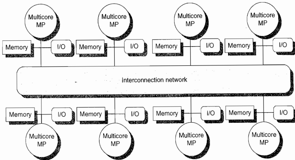
Figure 5.2 The basic architecture of a distributed-memory multiprocessor in 2011 typically consists of a multicore multiprocessor chip with memory and possibly I/O attached and an interface to an interconnection network that connects all the nodes. Each processor core shares the entire memory, although the access time to the local memory attached to the core's chip will be much faster than the access time to remote memories.
