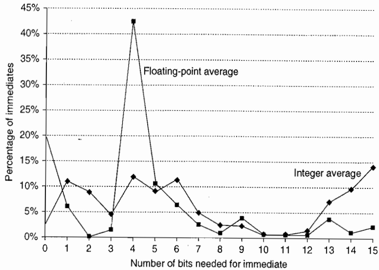
Figure A.10 The distribution of immediate values. The x -axis shows the number of bits needed to represent the magnitude of an immediate value—0 means the immediate field value was 0. The majority of the immediate values are positive. About 20% were negative for CINT2000, and about 30% were negative for CFP2000. These measurements were taken on an Alpha, where the maximum immediate is 16 bits, for the same programs as in Figure A.8. A similar measurement on the VAX, which supported 32-bit immediates, showed that about 20% to 25% of immediates were longer than 16 bits. Thus, 16 bits would capture about 80% and 8 bits about 50%.
