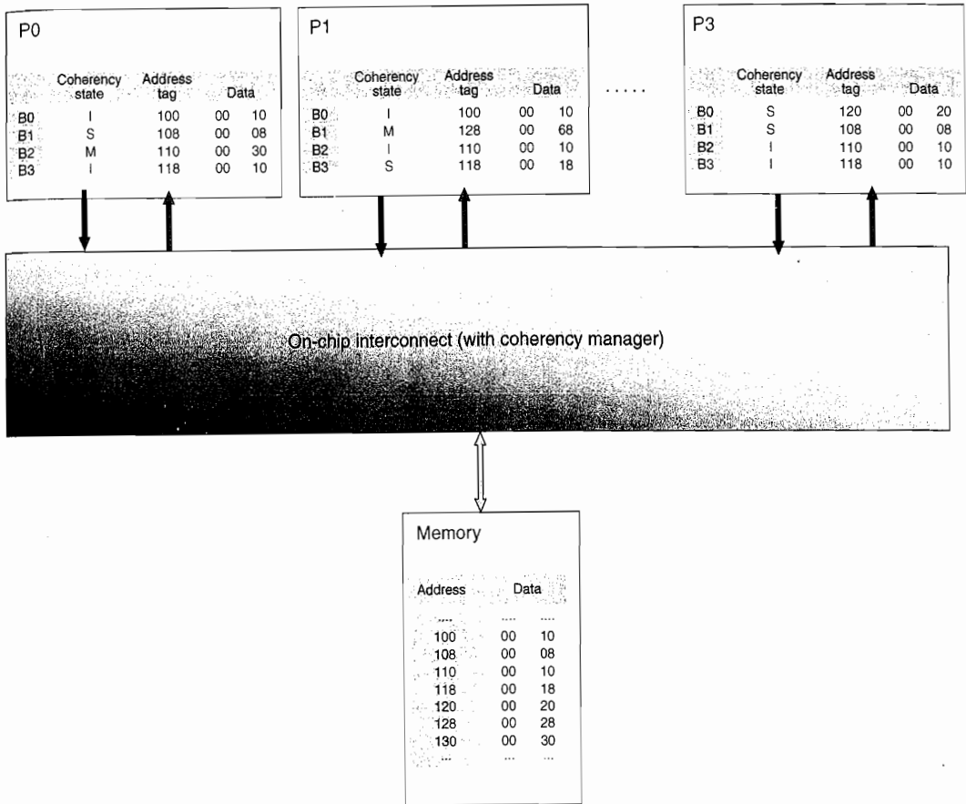
Figure 5.35 Multicore (point-to-point) multiprocessor.
