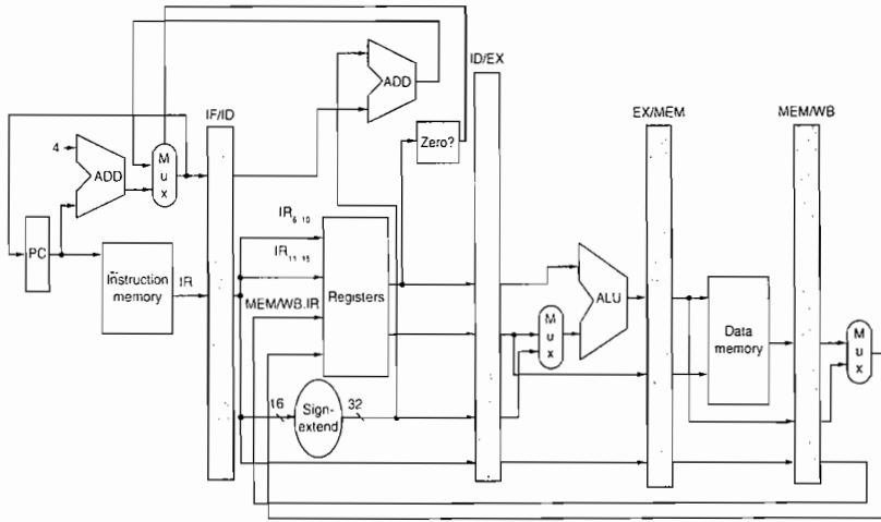
Figure C.28 The stall from branch hazards can be reduced by moving the zero test and branch-target calculation into the ID phase of the pipeline. Notice that we have made two important changes, each of which removes 1 cycle from the 3-cycle stall for branches. The first change is to move both the branch-target address calculation and the branch condition decision to the ID cycle. The second change is to write the PC of the instruction in the IF phase, using either the branch-target address computed during ID or the incremented PC computed during IF. In comparison, Figure C.22 obtained the branch-target address from the EX/MEM register and wrote the result during the MEM clock cycle. As mentioned in Figure C.22, the PC can be thought of as a pipeline register (e.g., as part of ID/IF), which is written with the address of the next instruction at the end of each IF cycle.
