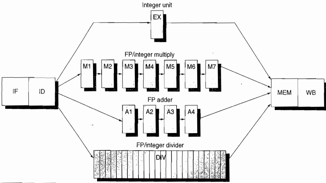
Figure C.35 A pipeline that supports multiple outstanding FP operations. The FP multiplier and adder are fully pipelined and have a depth of seven and four stages, respectively. The FP divider is not pipelined, but requires 24 clock cycles to complete. The latency in instructions between the issue of an FP operation and the use of the result of that operation without incurring a RAW stall is determined by the number of cycles spent in the execution stages. For example, the fourth instruction after an FP add can use the result of the FP add. For integer ALU operations, the depth of the execution pipeline is always one and the next instruction can use the results.
