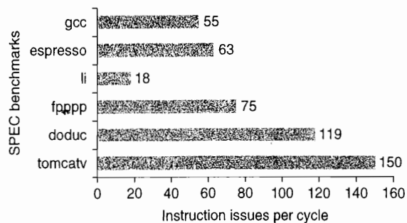
Figure 3.26 ILP available in a perfect processor for six of the SPEC92 benchmarks. The first three programs are integer programs, and the last three are floating-point programs. The floating-point programs are loop intensive and have large amounts of loop-level parallelism.
