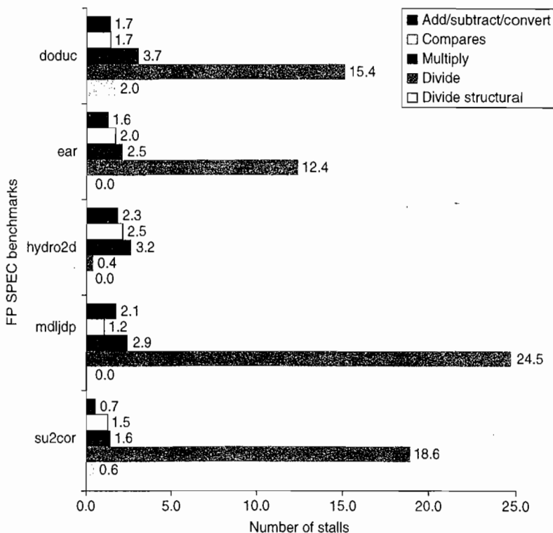
Figure C.39 Stalls per FP operation for each major type of FP operation for the SPEC89 FP benchmarks. Except for the divide structural hazards, these data do not depend on the frequency of an operation, only on its latency and the number of cycles before the result is used. The number of stalls from RAW hazards roughly tracks the latency of the FP unit. For example, the average number of stalls per FP add, subtract, or convert is 1.7 cycles, or 56% of the latency (3 cycles). Likewise, the average number of stalls for multiplies and divides are 2.8 and 14.2, respectively, or 46% and 59% of the corresponding latency. Structural hazards for divides are rare, since the divide frequency is low.
