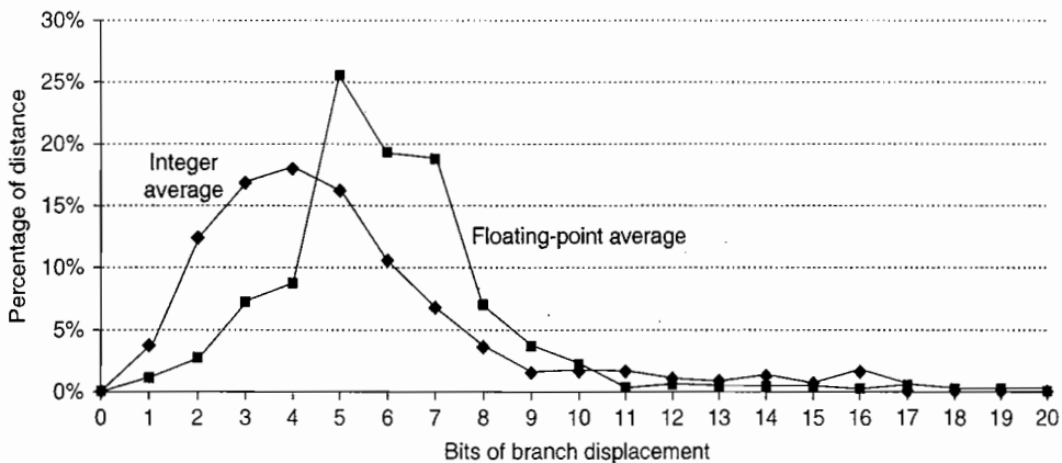
Figure A.15 Branch distances in terms of number of instructions between the target and the branch instruction. The most frequent branches in the integer programs are to targets that can be encoded in 4 to 8 bits. This result tells us that short displacement fields often suffice for branches and that the designer can gain some encoding density by having a shorter instruction with a smaller branch displacement. These measurements were taken on a load-store computer (Alpha architecture) with all instructions aligned on word boundaries. An architecture that requires fewer instructions for the same program, such as a VAX, would have shorter branch distances. However, the number of bits needed for the displacement may increase if the computer has variable-length instructions to be aligned on any byte boundary. The programs and computer used to collect these statistics are the same as those in Figure A.8.
