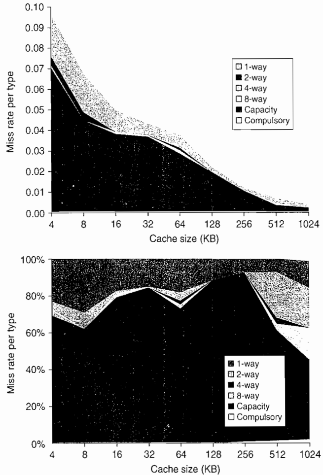
Figure B.9 Total miss rate (top) and distribution of miss rate (bottom) for each size cache according to the three C's for the data in Figure B.8. The top diagram shows the actual data cache miss rates, while the bottom diagram shows the percentage in each category. (Space allows the graphs to show one extra cache size than can fit in Figure B.8.)
