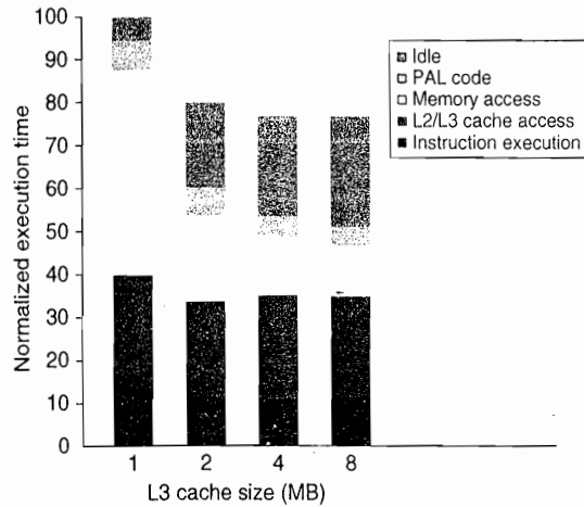
Figure 5.12 The relative performance of the OLTP workload as the size of the L3 cache, which is set as two-way set associative, grows from 1 MB to 8 MB. The idle time also grows as cache size is increased, reducing some of the performance gains. This growth occurs because, with fewer memory system stalls, more server processes are needed to cover the I/O latency. The workload could be retuned to increase the computation/communication balance, holding the idle time in check. The PAL code is a set of sequences of specialized OS-level instructions executed in privileged mode; an example is the TLB miss handler.
