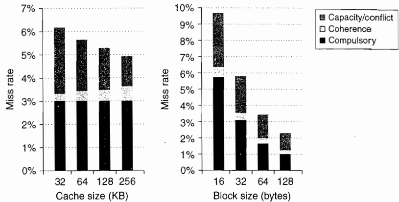
Figure 5.18 The components of the kernel data miss rate change as the L1 data cache size is increased from 32 KB to 256 KB, when the multiprocessing workload is run on eight processors. The compulsory miss rate component stays constant, since it is unaffected by cache size. The capacity component drops by more than a factor of 2, while the coherence component nearly doubles. The increase in coherence misses occurs because the probability of a miss being caused by an invalidation increases with cache size, since fewer entries are bumped due to capacity. As we would expect, the increasing block size of the L1 data cache substantially reduces the compulsory miss rate in the kernel references. It also has a significant impact on the capacity miss rate, decreasing it by a factor of 2.4 over the range of block sizes. The increased block size has a small reduction in coherence traffic, which appears to stabilize at 64 bytes, with no change in the coherence miss rate in going to 128-byte lines. Because there are no significant reductions in the coherence miss rate as the block size increases, the fraction of the miss rate due to coherence grows from about 7% to about 15%.
