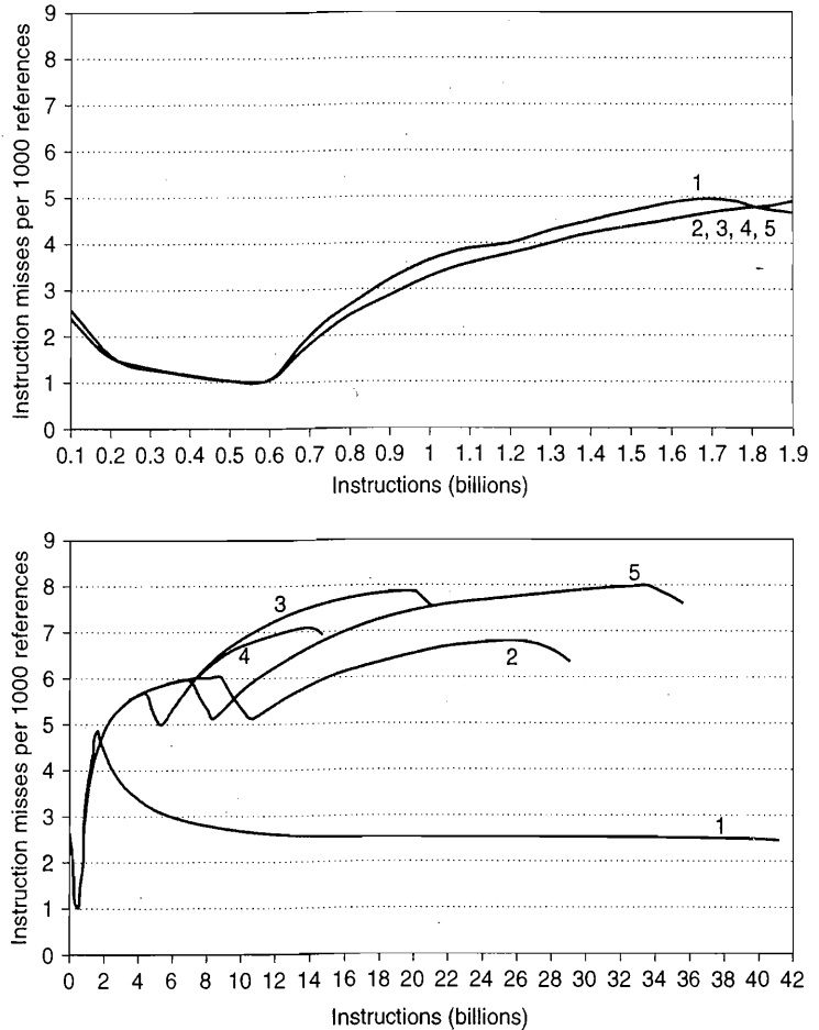
Figure 2.27 Instruction misses per 1000 references for five inputs to the perl benchmark from SPEC2000. There is little variation in misses and little difference between the five inputs for the first 1.9 billion instructions. Running to completion shows how misses vary over the life of the program and how they depend on the input. The top graph shows the running average misses for the first 1.9 billion instructions, which starts at about 2.5 and ends at about 4.7 misses per 1000 references for all five inputs. The bottom graph shows the running average misses to run to completion, which takes 16 to 41 billion instructions depending on the input. After the first 1.9 billion instructions, the misses per 1000 references vary from 2.4 to 7.9 depending on the input. The simulations were for the Alpha processor using separate L1 caches for instructions and data, each two-way 64 KB with LRU, and a unified 1 MB direct-mapped L2 cache.
