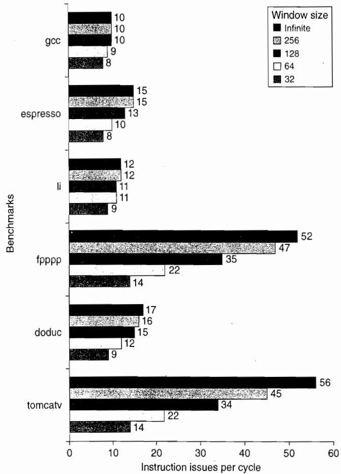
Figure 3.27 The amount of parallelism available versus the window size for a variety of integer and floating-point programs with up to 64 arbitrary instruction issues per clock. Although there are fewer renaming registers than the window size, the fact that all operations have one-cycle latency and the number of renaming registers equals the issue width allows the processor to exploit parallelism within the entire window. In a real implementation, the window size and the number of renaming registers must be balanced to prevent one of these factors from overly constraining the issue rate.
