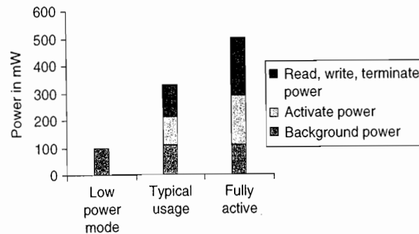
Figure 2.15 Power consumption for a DDR3 SDRAM operating under three conditions: low power (shutdown) mode, typical system mode (DRAM is active 30% of the time for reads and 15% for writes), and fully active mode, where the DRAM is continuously reading or writing when not in precharge. Reads and writes assume bursts of 8 transfers. These data are based on a Micron 1.5V 2Gb DDR3-1066.
