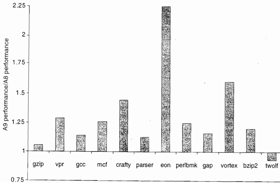
Figure 3.40 The performance ratio for the A9 compared to the A8, both using a 1 GHz clock and the same size caches for L1 and L2, shows that the A9 is about 1.28 times faster. Both runs use a 32 KB primary cache and a 1 MB secondary cache, which is 8-way set associative for the A8 and 16-way for the A9. The block sizes in the caches are 64 bytes for the A8 and 32 bytes for the A9. As mentioned in the caption of Figure 3.39, eon makes intensive use of integer multiply, and the combination of dynamic scheduling and a faster multiply pipeline significantly improves performance on the A9. twolf experiences a small slowdown, likely due to the fact that its cache behavior is worse with the smaller L1 block size of the A9.
