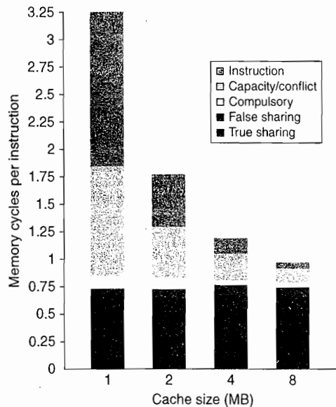
Figure 5.13 The contributing causes of memory access cycle shift as the cache size is increased. The L3 cache is simulated as two-way set associative.
