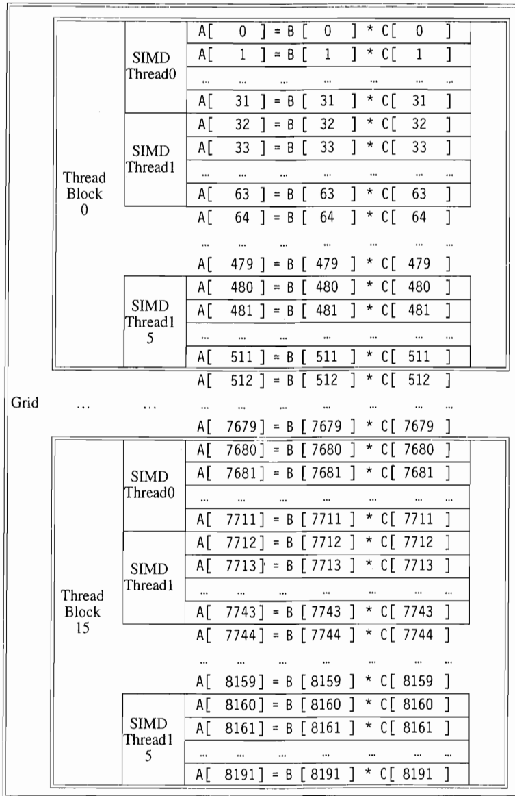
Figure 4.13 The mapping of a Grid (vectorizable loop), Thread Blocks (SIMD basic blocks), and threads of SIMD instructions to a vector-vector multiply, with each vector being 8192 elements long. Each thread of SIMD instructions calculates 32 elements per instruction, and in this example each Thread Block contains 16 threads of SIMD instructions and the Grid contains 16 Thread Blocks. The hardware Thread Block Scheduler assigns Thread Blocks to multithreaded SIMD Processors and the hardware Thread Scheduler picks which thread of SIMD instructions to run each clock cycle within a SIMD Processor. Only SIMD Threads in the same Thread Block can communicate via Local Memory. (The maximum number of SIMD Threads that can execute simultaneously per Thread Block is 16 for Tesla-generation GPUs and 32 for the later Fermi-generation GPUs.)
