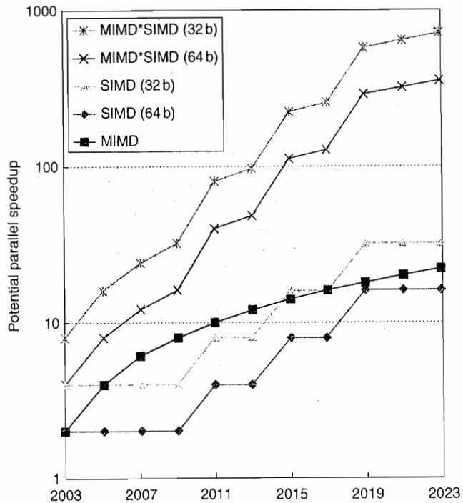
Figure 4.1 Potential speedup via parallelism from MIMD, SIMD, and both MIMD and SIMD over time for x86 computers. This figure assumes that two cores per chip for MIMD will be added every two years and the number of operations for SIMD will double every four years.
