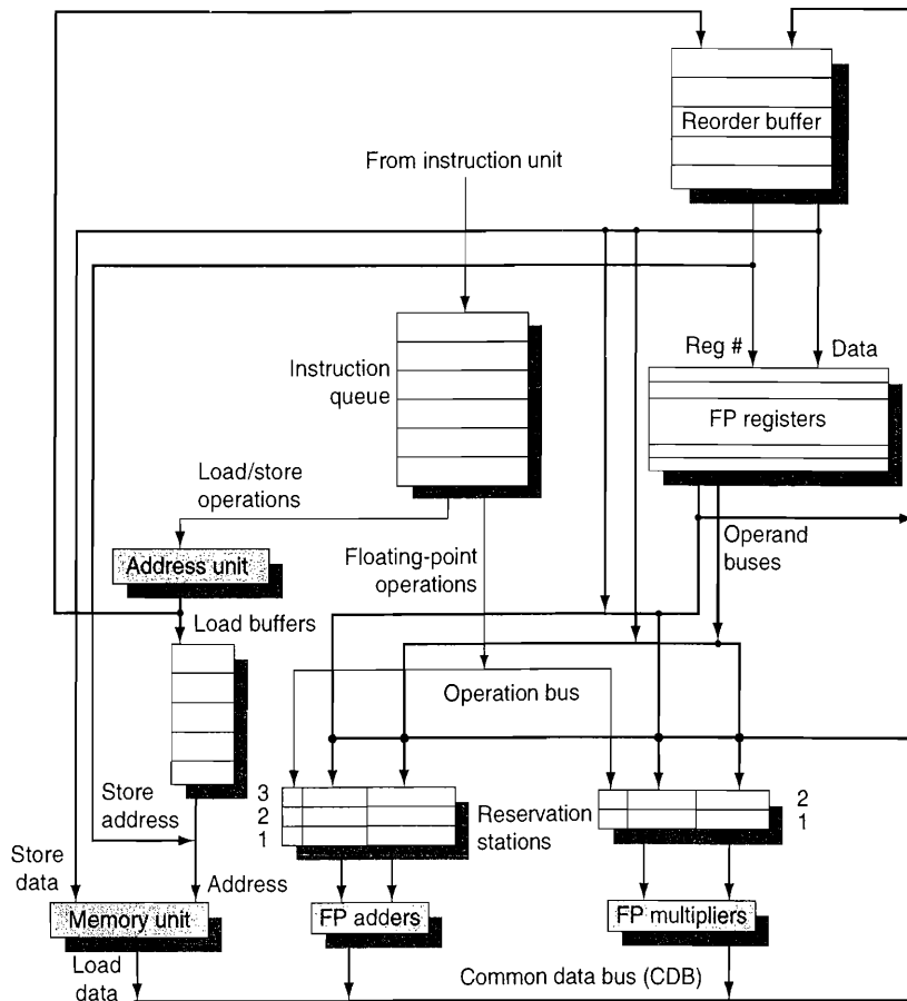
Figure 3.11 The basic structure of a FP unit using Tomasulo's algorithm and extended to handle speculation. Comparing this to Figure 3.6 on page 173, which implemented Tomasulo's algorithm, the major change is the addition of the ROB and the elimination of the store buffer, whose function is integrated into the ROB. This mechanism can be extended to multiple issue by making the CDB wider to allow for multiple completions per clock.
