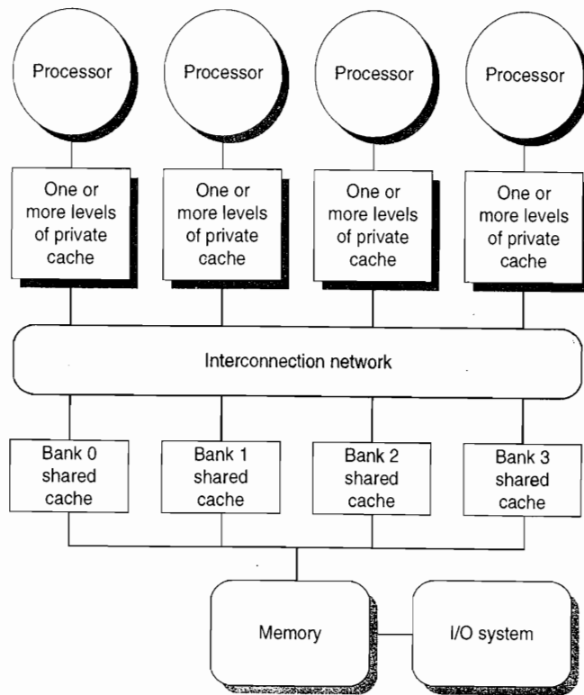
Figure 5.8 A multicore single-chip multiprocessor with uniform memory access through a banked shared cache and using an interconnection network rather than a bus.
