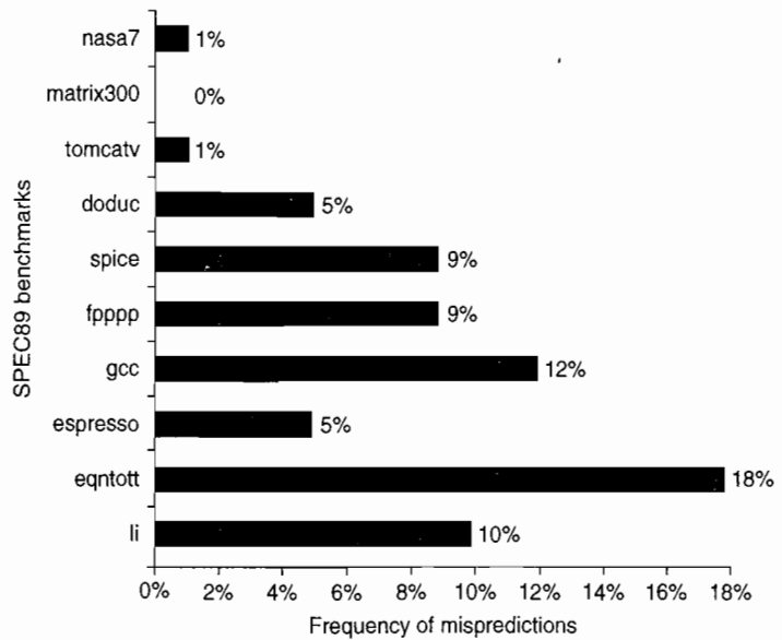
Figure C.19 Prediction accuracy of a 4096-entry 2-bit prediction buffer for the SPEC89 benchmarks. The misprediction rate for the integer benchmarks (gcc, espresso, eqntott, and li) is substantially higher (average of 11%) than that for the floating-point programs (average of 4%). Omitting the floating-point kernels (nasa7, matrix300, and tomcatv) still yields a higher accuracy for the FP benchmarks than for the integer benchmarks. These data, as well as the rest of the data in this section, are taken from a branch-prediction study done using the IBM Power architecture and optimized code for that system. See Pan, So, and Rameh [1992]. Although these data are for an older version of a subset of the SPEC benchmarks, the newer benchmarks are larger and would show slightly worse behavior, especially for the integer benchmarks.
