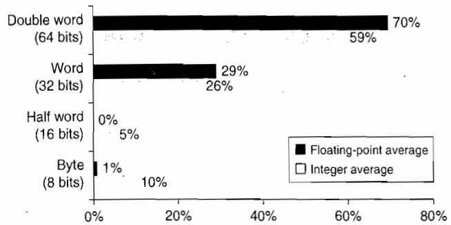
Figure A.11 Distribution of data accesses by size for the benchmark programs. The double-word data type is used for double-precision floating point in floating-point programs and for addresses, since the computer uses 64-bit addresses. On a 32-bit address computer the 64-bit addresses would be replaced by 32-bit addresses, and so almost all double-word accesses in integer programs would become single-word accesses.
