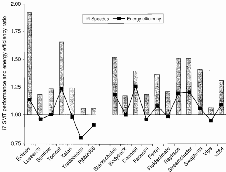
Figure 3.35 The speedup from using multithreading on one core on an i7 processor averages 1.28 for the Java benchmarks and 1.31 for the PARSEC benchmarks (using an unweighted harmonic mean, which implies a workload where the total time spent executing each benchmark in the single-threaded base set was the same). The energy efficiency averages 0.99 and 1.07, respectively (using the harmonic mean). Recall that anything above 1.0 for energy efficiency indicates that the feature reduces execution time by more than it increases average power. Two of the Java benchmarks experience little speedup and have significant negative energy efficiency because of this. Turbo Boost is off in all cases. These data were collected and analyzed by Esmaeilzadeh et al. [2011] using the Oracle (Sun) HotSpot build 16.3-b01 Java 1.6.0 Virtual Machine and the gcc v4.4.1 native compiler.
