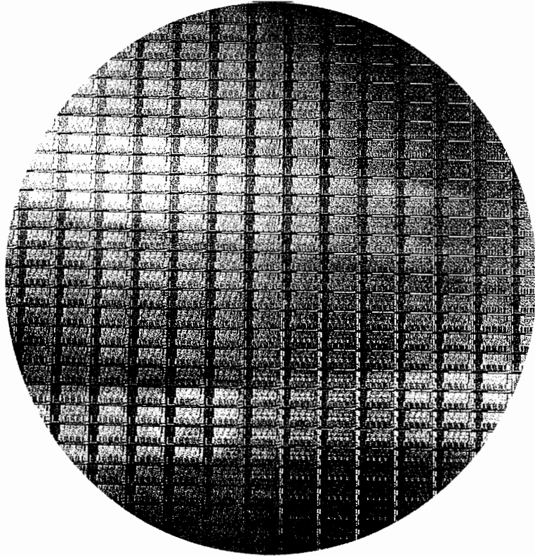
Figure 1.15 This 300 mm wafer contains 280 full Sandy Bridge dies, each 20.7 by 10.5 mm in a 32 nm process. (Sandy Bridge is Intel's successor to Nehalem used in the Core i7.) At 216 mm 2 , the formula for dies per wafer estimates 282. (Courtesy Intel.)
