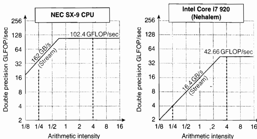
Figure 4.11 Roofline model for one NEC SX-9 vector processor on the left and the Intel Core i7 920 multicore computer with SIMD Extensions on the right [Williams et al. 2009]. This Roofline is for unit-stride memory accesses and double-precision floating-point performance. NEC SX-9 is a vector supercomputer announced in 2008 that costs millions of dollars. It has a peak DP FP performance of 102.4 GFLOP/sec and a peak memory bandwidth of 162 GBytes/sec from the Stream benchmark. The Core i7 920 has a peak DP FP performance of 42.66 GFLOP/sec and a peak memory bandwidth of 16.4 GBytes/sec. The dashed vertical lines at an arithmetic intensity of 4 FLOP/byte show that both processors operate at peak performance. In this case, the SX-9 at 102.4 FLOP/sec is 2.4× faster than the Core i7 at 42.66 GFLOP/sec. At an arithmetic intensity of 0.25 FLOP/byte, the SX-9 is 10× faster at 40.5 GFLOP/sec versus 4.1 GFLOP/sec for the Core i7.
