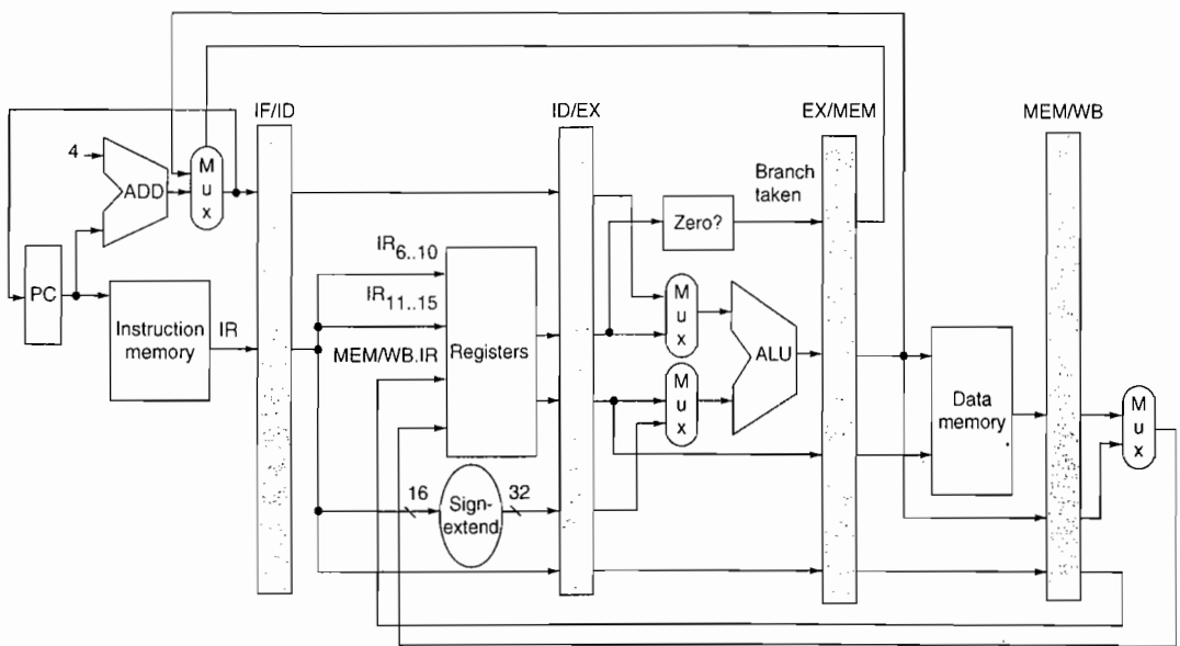
Figure C.22 The data path is pipelined by adding a set of registers, one between each pair of pipe stages. The registers serve to convey values and control information from one stage to the next. We can also think of the PC as a pipeline register, which sits before the IF stage of the pipeline, leading to one pipeline register for each pipe stage. Recall that the PC is an edge-triggered register written at the end of the clock cycle; hence, there is no race condition in writing the PC. The selection multiplexer for the PC has been moved so that the PC is written in exactly one stage (IF). If we didn't move it, there would be a conflict when a branch occurred, since two instructions would try to write different values into the PC. Most of the data paths flow from left to right, which is from earlier in time to later. The paths flowing from right to left (which carry the register write-back information and PC information on a branch) introduce complications into our pipeline.
