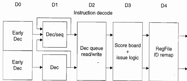
Figure 3.37 The five-stage instruction decode of the A8. In the first stage, a PC produced by the fetch unit (either from the branch target buffer or the PC incremter) is used to retrieve an 8-byte block from the cache. Up to two instructions are decoded and placed into the decode queue; if neither instruction is a branch, the PC is incremented for the next fetch. Once in the decode queue, the scoreboard logic decides when the instructions can issue. In the issue, the register operands are read; recall that in a simple scoreboard, the operands always come from the registers. The register operands and opcode are sent to the instruction execution portion of the pipeline.
