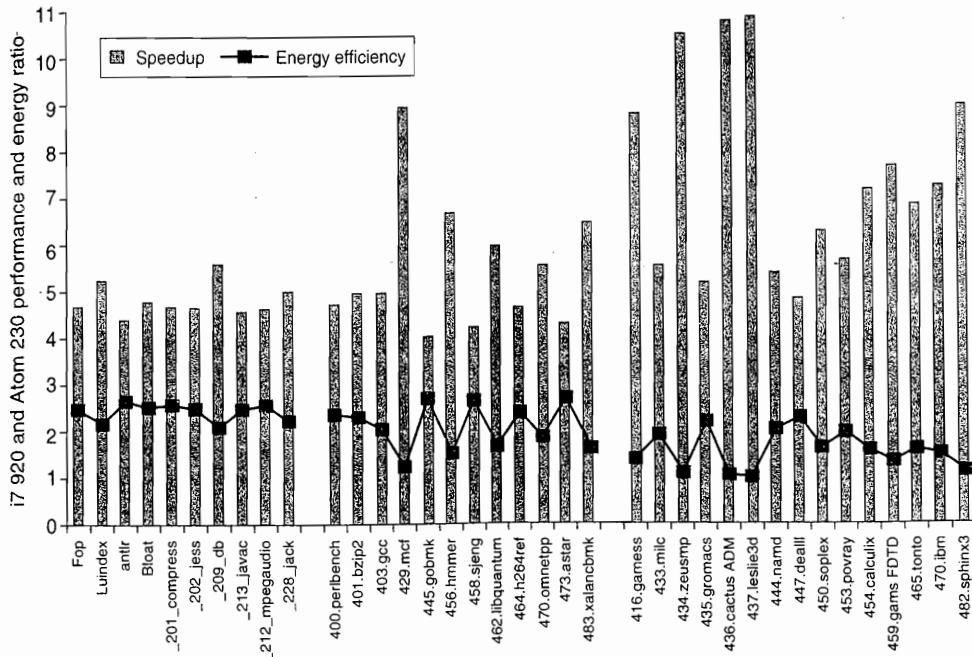
Figure 3.45 The relative performance and energy efficiency for a set of single-threaded benchmarks shows the i7 920 is 4 to over 10 times faster than the Atom 230 but that it is about 2 times less power efficient on average! Performance is shown in the columns as i7 relative to Atom, which is execution time (i7)/execution time (Atom). Energy is shown with the line as Energy (Atom)/Energy (i7). The i7 never beats the Atom in energy efficiency, although it is essentially as good on four benchmarks, three of which are floating point. The data shown here were collected by Esmaeilzadeh et al. [2011]. The SPEC benchmarks were compiled with optimization on using the standard Intel compiler, while the Java benchmarks use the Sun (Oracle) Hotspot Java VM. Only one core is active on the i7, and the rest are in deep power saving mode. Turbo Boost is used on the i7, which increases its performance advantage but slightly decreases its relative energy efficiency.
