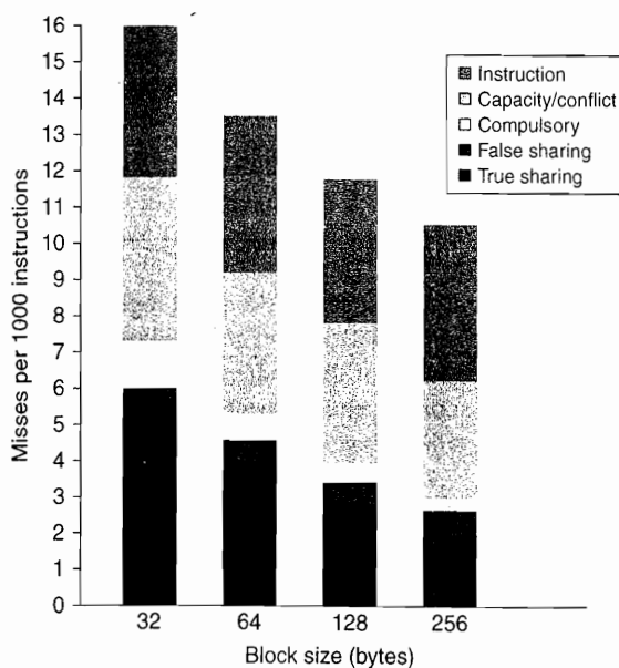
Figure 5.15 The number of misses per 1000 instructions drops steadily as the block size of the L3 cache is increased, making a good case for an L3 block size of at least 128 bytes. The L3 cache is 2 MB, two-way set associative.
