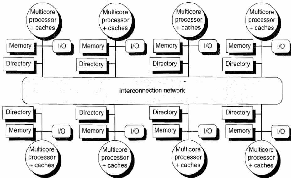
Figure 5.20 A directory is added to each node to implement cache coherence in a distributed-memory multiprocessor. In this case, a node is shown as a single multicore chip, and the directory information for the associated memory may reside either on or off the multicore. Each directory is responsible for tracking the caches that share the memory addresses of the portion of memory in the node. The coherence mechanism would handle both the maintenance of the directory information and any coherence actions needed within the multicore node.
