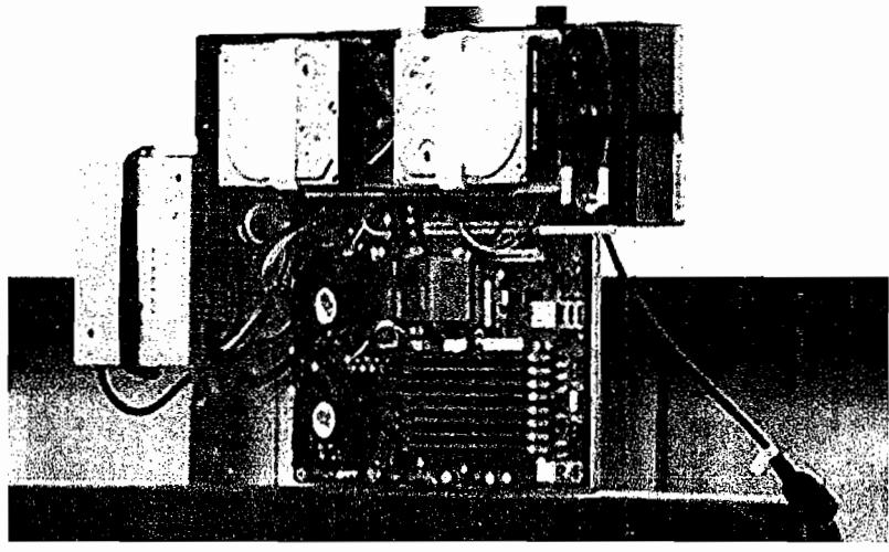
Figure 6.21 Server for Google WSC. The power supply is on the left and the two disks are on the top. The two fans below the left disk cover the two sockets of the AMD Barcelona microprocessor, each with two cores, running at 2.2 GHz. The eight DIMMs in the lower right each hold 1 GB, giving a total of 8 GB. There is no extra sheet metal, as the servers are plugged into the battery and a separate plenum is in the rack for each server to help control the airflow. In part because of the height of the batteries, 20 servers fit in a rack.
