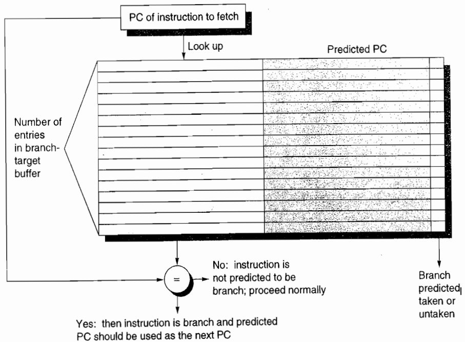
Figure 3.21 A branch-target buffer. The PC of the instruction being fetched is matched against a set of instruction addresses stored in the first column; these represent the addresses of known branches. If the PC matches one of these entries, then the instruction being fetched is a taken branch, and the second field, predicted PC, contains the prediction for the next PC after the branch. Fetching begins immediately at that address. The third field, which is optional, may be used for extra prediction state bits.
