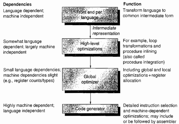
Figure A.19 Compilers typically consist of two to four passes, with more highly optimizing compilers having more passes. This structure maximizes the probability that a program compiled at various levels of optimization will produce the same output when given the same input. The optimizing passes are designed to be optional and may be skipped when faster compilation is the goal and lower-quality code is acceptable. A pass is simply one phase in which the compiler reads and transforms the entire program. (The term phase is often used interchangeably with pass .) Because the optimizing passes are separated, multiple languages can use the same optimizing and code generation passes. Only a new front end is required for a new language.
