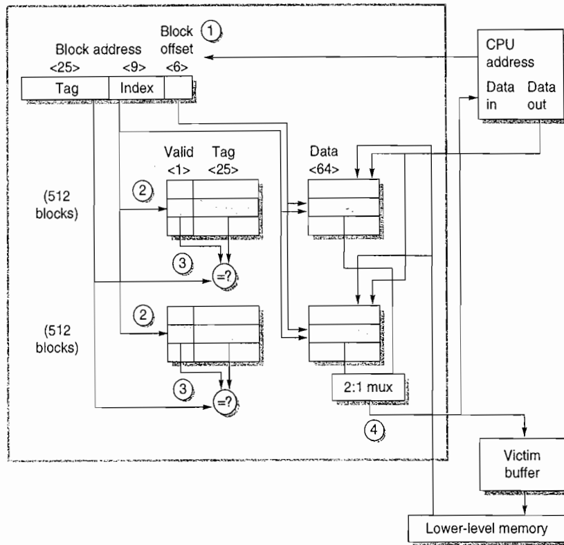
Figure B.5 The organization of the data cache in the Opteron microprocessor. The 64 KB cache is two-way set associative with 64-byte blocks. The 9-bit index selects among 512 sets. The four steps of a read hit, shown as circled numbers in order of occurrence, label this organization. Three bits of the block offset join the index to supply the RAM address to select the proper 8 bytes. Thus, the cache holds two groups of 4096 64-bit words, with each group containing half of the 512 sets. Although not exercised in this example, the line from lower-level memory to the cache is used on a miss to load the cache. The size of address leaving the processor is 40 bits because it is a physical address and not a virtual address. Figure B.24 on page B-47 explains how the Opteron maps from virtual to physical for a cache access.
