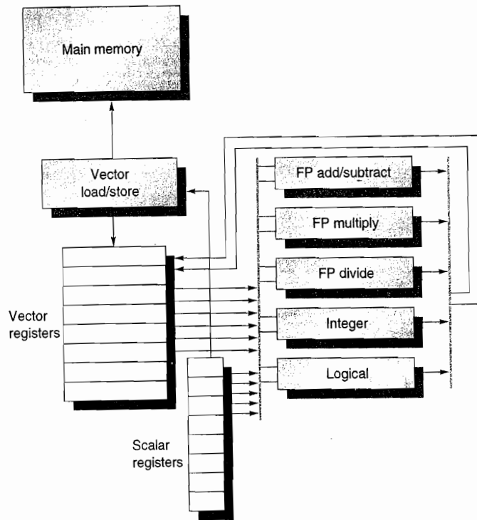
Figure 4.2 The basic structure of a vector architecture, VMIPS. This processor has a scalar architecture just like MIPS. There are also eight 64-element vector registers, and all the functional units are vector functional units. This chapter defines special vector instructions for both arithmetic and memory accesses. The figure shows vector units for logical and integer operations so that VMIPS looks like a standard vector processor that usually includes these units; however, we will not be discussing these units. The vector and scalar registers have a significant number of read and write ports to allow multiple simultaneous vector operations. A set of crossbar switches (thick gray lines) connects these ports to the inputs and outputs of the vector functional units.
