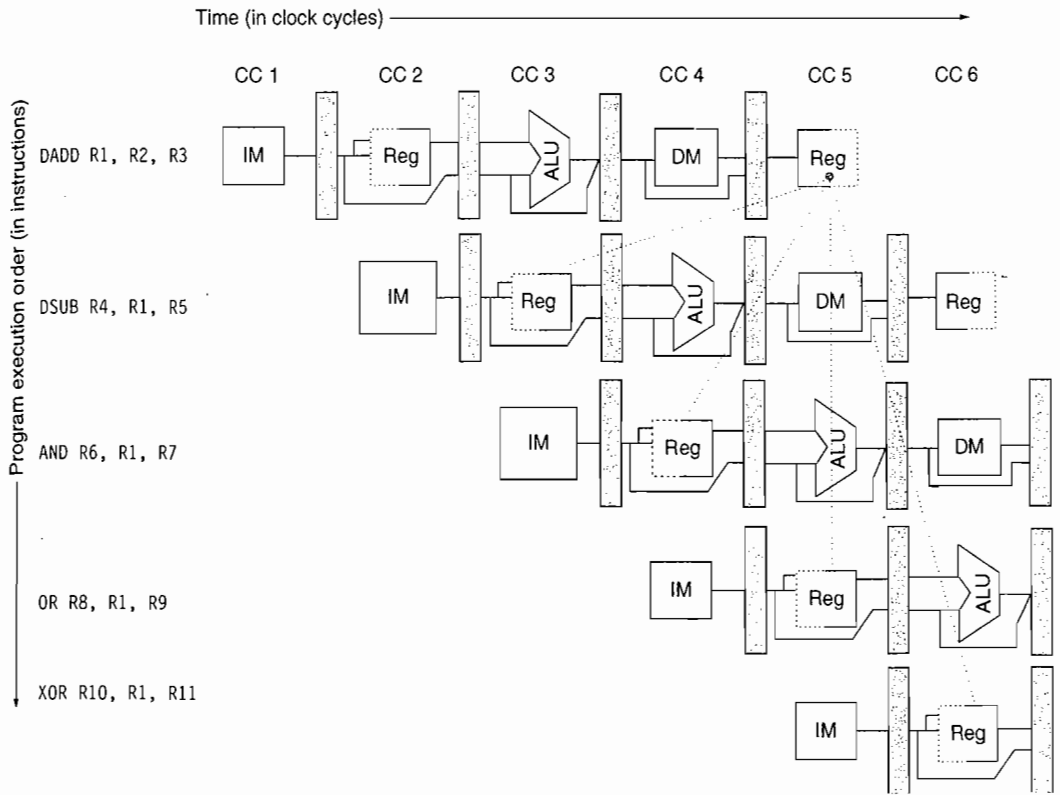
Figure C.6 The use of the result of the DADD instruction in the next three instructions causes a hazard, since the register is not written until after those instructions read it.
