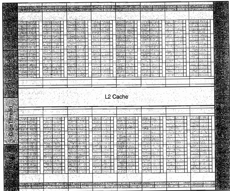
Figure 4.15 Floor plan of the Fermi GTX 480 GPU. This diagram shows 16 multi-threaded SIMD Processors. The Thread Block Scheduler is highlighted on the left. The GTX 480 has 6 GDDR5 ports, each 64 bits wide, supporting up to 6 GB of capacity. The Host Interface is PCI Express 2.0 x 16. Giga Thread is the name of the scheduler that distributes thread blocks to Multiprocessors, each of which has its own SIMD Thread Scheduler.
