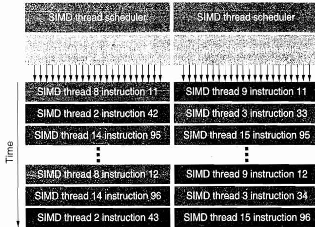
Figure 4.19 Block Diagram of Fermi's Dual SIMD Thread Scheduler. Compare this design to the single SIMD Thread Design in Figure 4.16.
