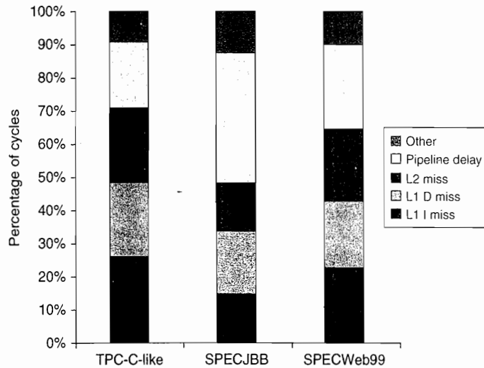
Figure 3.32 The breakdown of causes for a thread being not ready. The contribution to the “other” category varies. In TPC-C, store buffer full is the largest contributor; in SPEC-JBB, atomic instructions are the largest contributor; and in SPECWeb99, both factors contribute.
