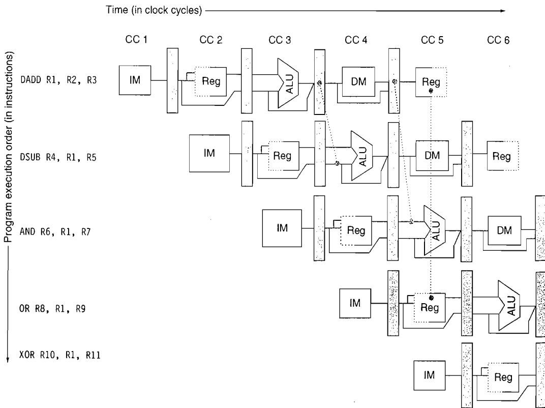
Figure C.7 A set of instructions that depends on the DADD result uses forwarding paths to avoid the data hazard. The inputs for the DSUB and AND instructions forward from the pipeline registers to the first ALU input. The OR receives its result by forwarding through the register file, which is easily accomplished by reading the registers in the second half of the cycle and writing in the first half, as the dashed lines on the registers indicate. Notice that the forwarded result can go to either ALU input; in fact, both ALU inputs could use forwarded inputs from either the same pipeline register or from different pipeline registers. This would occur, for example, if the AND instruction was AND R6, R1, R4.
