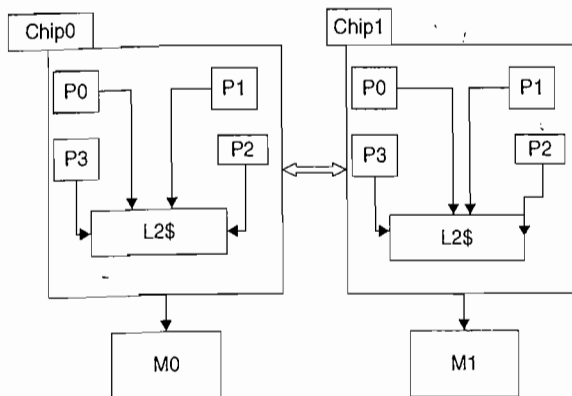
Figure 5.37 Multichip, multicore multiprocessor with DSM.
