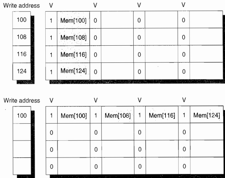
Figure 2.7 To illustrate write merging, the write buffer on top does not use it while the write buffer on the bottom does. The four writes are merged into a single buffer entry with write merging; without it, the buffer is full even though three-fourths of each entry is wasted. The buffer has four entries, and each entry holds four 64-bit words. The address for each entry is on the left, with a valid bit (V) indicating whether the next sequential 8 bytes in this entry are occupied. (Without write merging, the words to the right in the upper part of the figure would only be used for instructions that wrote multiple words at the same time.)
