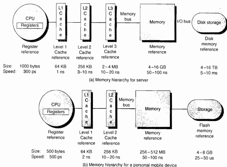
Figure 2.1 The levels in a typical memory hierarchy in a server computer shown on top (a) and in a personal mobile device (PMD) on the bottom (b). As we move farther away from the processor, the memory in the level below becomes slower and larger. Note that the time units change by a factor of 10^9 —from picoseconds to milliseconds—and that the size units change by a factor of 10^{12} —from bytes to terabytes. The PMD has a slower clock rate and smaller caches and main memory. A key difference is that servers and desktops use disk storage as the lowest level in the hierarchy while PMDs use Flash, which is built from EEPROM technology.
