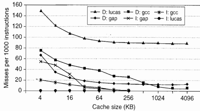
Figure 2.26 Instruction and data misses per 1000 instructions as cache size varies from 4 KB to 4096 KB. Instruction misses for gcc are 30,000 to 40,000 times larger than lucas, and, conversely, data misses for lucas are 2 to 60 times larger than gcc. The programs gap, gcc, and lucas are from the SPEC2000 benchmark suite.
