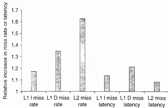
Figure 3.30 The relative change in the miss rates and miss latencies when executing with one thread per core versus four threads per core on the TPC-C benchmark. The latencies are the actual time to return the requested data after a miss. In the four-thread case, the execution of other threads could potentially hide much of this latency.
