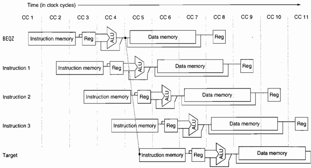
Figure C.44 The basic branch delay is 3 cycles, since the condition evaluation is performed during EX.
