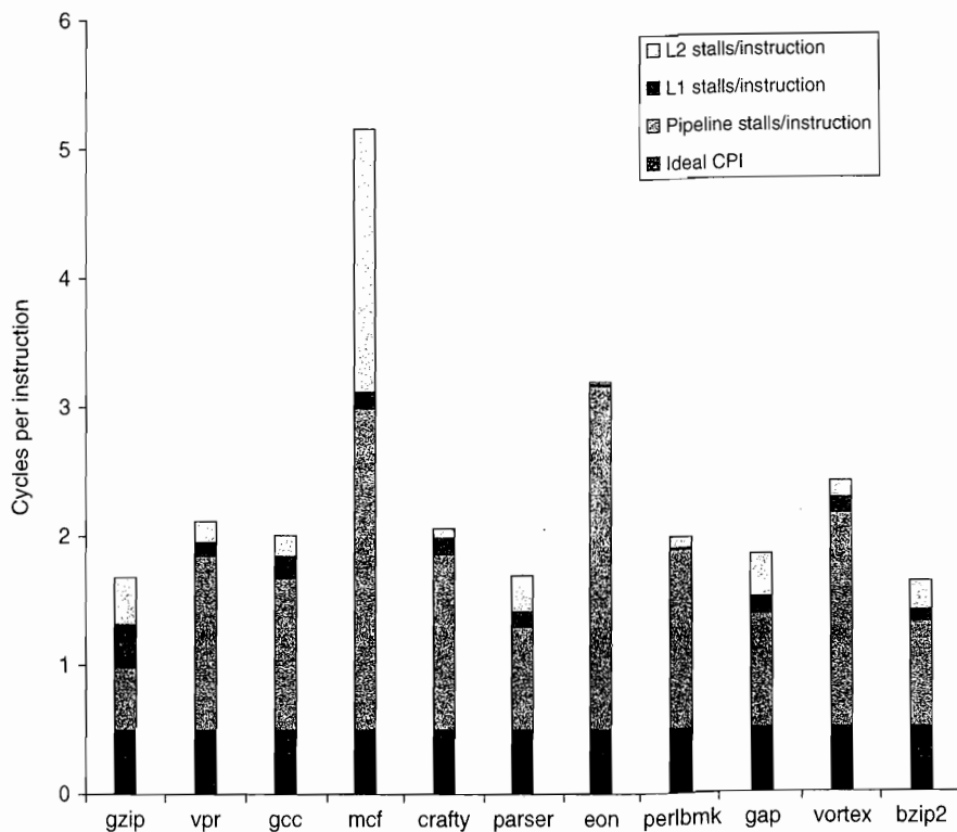
Figure 3.39 The estimated composition of the CPI on the ARM A8 shows that pipeline stalls are the primary addition to the base CPI. eon deserves some special mention, as it does integer-based graphics calculations (ray tracing) and has very few cache misses. It is computationally intensive with heavy use of multiples, and the single multiply pipeline becomes a major bottleneck. This estimate is obtained by using the L1 and L2 miss rates and penalties to compute the L1 and L2 generated stalls per instruction. These are subtracted from the CPI measured by a detailed simulator to obtain the pipeline stalls. Pipeline stalls include all three hazards plus minor effects such as way misprediction.
