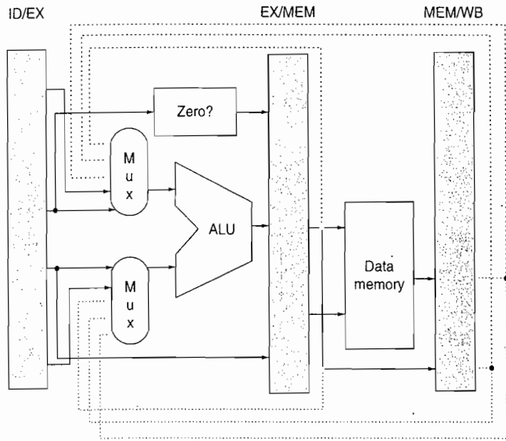
Figure C.27 Forwarding of results to the ALU requires the addition of three extra inputs on each ALU multiplexer and the addition of three paths to the new inputs. The paths correspond to a bypass of: (1) the ALU output at the end of the EX, (2) the ALU output at the end of the MEM stage, and (3) the memory output at the end of the MEM stage.
