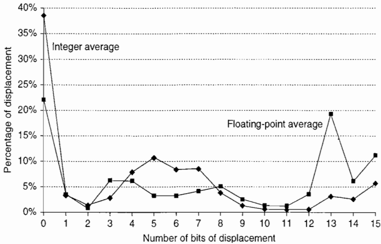
Figure A.8 Displacement values are widely distributed. There are both a large number of small values and a fair number of large values. The wide distribution of displacement values is due to multiple storage areas for variables and different displacements to access them (see Section A.8) as well as the overall addressing scheme the compiler uses. The x-axis is \log_2 of the displacement, that is, the size of a field needed to represent the magnitude of the displacement. Zero on the x-axis shows the percentage of displacements of value 0. The graph does not include the sign bit, which is heavily affected by the storage layout. Most displacements are positive, but a majority of the largest displacements (14+ bits) are negative. Since these data were collected on a computer with 16-bit displacements, they cannot tell us about longer displacements. These data were taken on the Alpha architecture with full optimization (see Section A.8) for SPEC CPU2000, showing the average of integer programs (CINT2000) and the average of floating-point programs (CFP2000).
