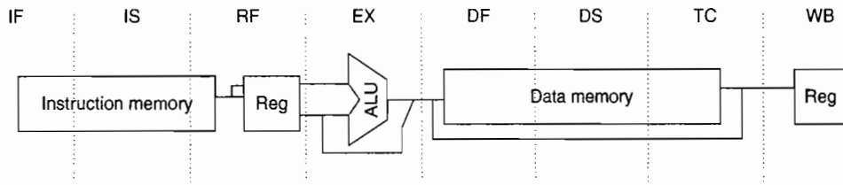
Figure C.41 The eight-stage pipeline structure of the R4000 uses pipelined instruction and data caches. The pipe stages are labeled and their detailed function is described in the text. The vertical dashed lines represent the stage boundaries as well as the location of pipeline latches. The instruction is actually available at the end of IS, but the tag check is done in RF, while the registers are fetched. Thus, we show the instruction memory as operating through RF. The TC stage is needed for data memory access, since we cannot write the data into the register until we know whether the cache access was a hit or not.
