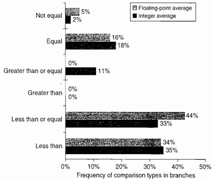
Figure A.17 Frequency of different types of compares in conditional branches. Less than (or equal) branches dominate this combination of compiler and architecture. These measurements include both the integer and floating-point compares in branches. The programs and computer used to collect these statistics are the same as those in Figure A.8.
