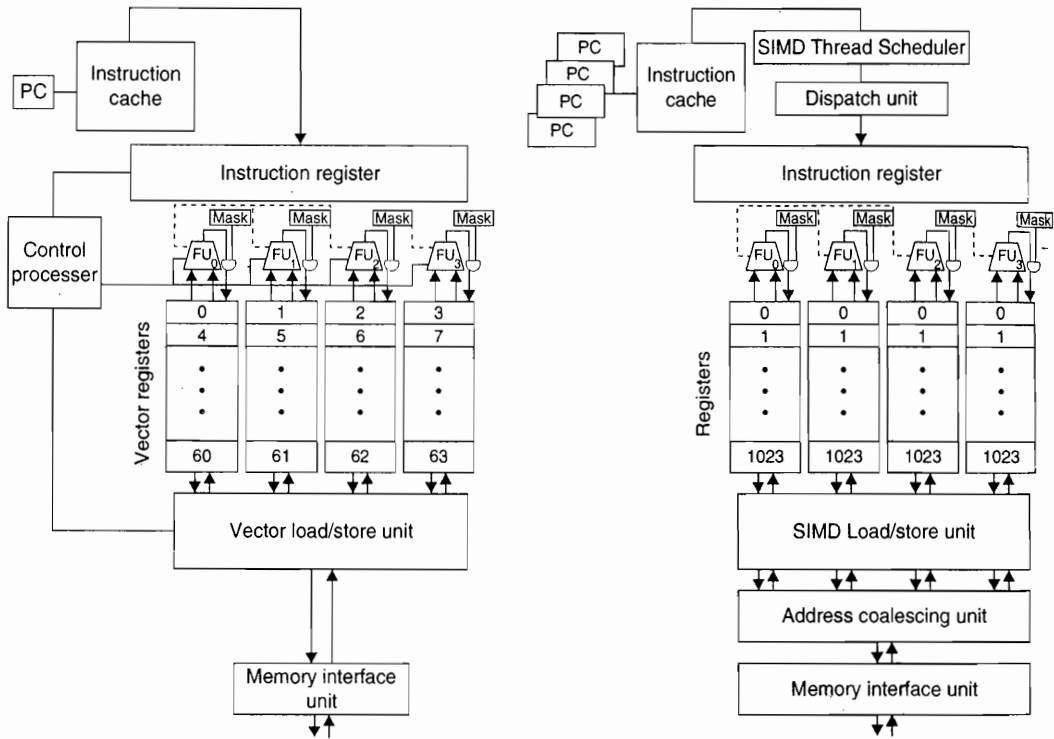
Figure 4.22 A vector processor with four lanes on the left and a multithreaded SIMD Processor of a GPU with four SIMD Lanes on the right. (GPUs typically have 8 to 16 SIMD Lanes.) The control processor supplies scalar operands for scalar-vector operations, increments addressing for unit and non-unit stride accesses to memory, and performs other accounting-type operations. Peak memory performance only occurs in a GPU when the Address Coalescing unit can discover localized addressing. Similarly, peak computational performance occurs when all internal mask bits are set identically. Note that the SIMD Processor has one PC per SIMD thread to help with multithreading.
