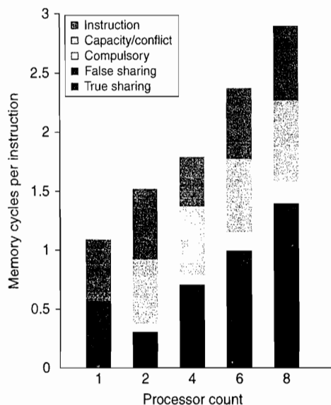
Figure 5.14 The contribution to memory access cycles increases as processor count increases primarily due to increased true sharing. The compulsory misses slightly increase since each processor must now handle more compulsory misses.
