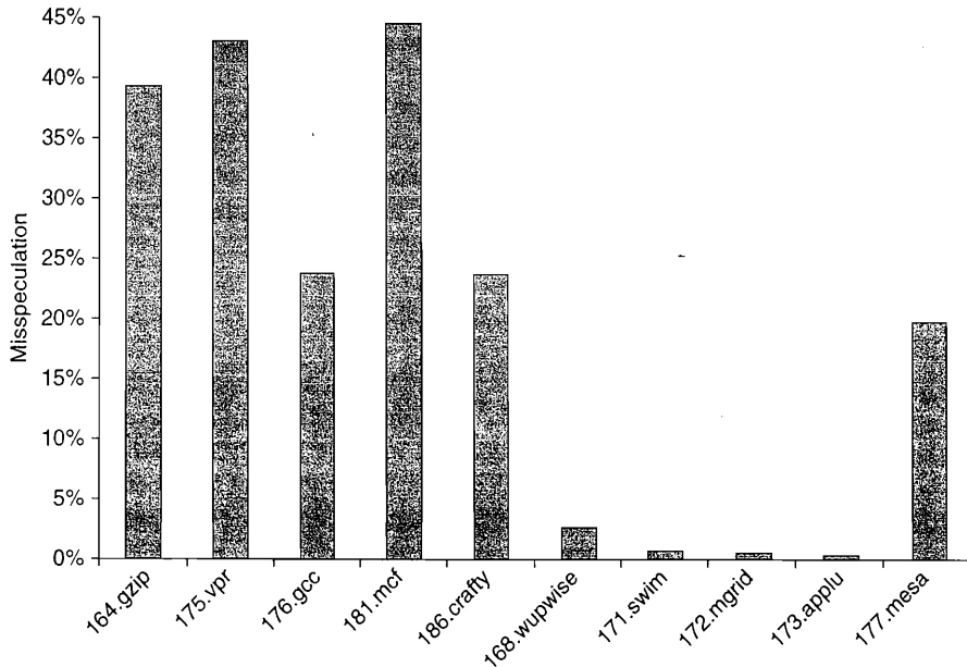
Figure 3.25 The fraction of instructions that are executed as a result of misspeculation is typically much higher for integer programs (the first five) versus FP programs (the last five).
