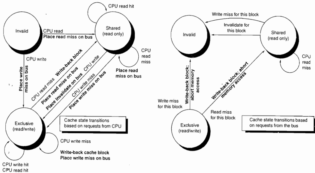
Figure 5.6 A write invalidate, cache coherence protocol for a private write-back cache showing the states and state transitions for each block in the cache. The cache states are shown in circles, with any access permitted by the local processor without a state transition shown in parentheses under the name of the state. The stimulus causing a state change is shown on the transition arcs in regular type, and any bus actions generated as part of the state transition are shown on the transition arc in bold. The stimulus actions apply to a block in the private cache, not to a specific address in the cache. Hence, a read miss to a block in the shared state is a miss for that cache block but for a different address. The left side of the diagram shows state transitions based on actions of the processor associated with this cache; the right side shows transitions based on operations on the bus. A read miss in the exclusive or shared state and a write miss in the exclusive state occur when the address requested by the processor does not match the address in the local cache block. Such a miss is a standard cache replacement miss. An attempt to write a block in the shared state generates an invalidate. Whenever a bus transaction occurs, all private caches that contain the cache block specified in the bus transaction take the action dictated by the right half of the diagram. The protocol assumes that memory (or a shared cache) provides data on a read miss for a block that is clean in all local caches. In actual implementations, these two sets of state diagrams are combined. In practice, there are many subtle variations on invalidate protocols, including the introduction of the exclusive unmodified state, as to whether a processor or memory provides data on a miss. In a multicore chip, the shared cache (usually L3, but sometimes L2) acts as the equivalent of memory, and the bus is the bus between the private caches of each core and the shared cache, which in turn interfaces to the memory.
