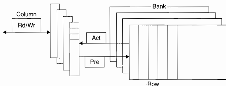
Figure 2.12 Internal organization of a DRAM. Modern DRAMs are organized in banks, typically four for DDR3. Each bank consists of a series of rows. Sending a PRE (pre-charge) command opens or closes a bank. A row address is sent with an Act (activate), which causes the row to transfer to a buffer. When the row is in the buffer, it can be transferred by successive column addresses at whatever the width of the DRAM is (typically 4, 8, or 16 bits in DDR3) or by specifying a block transfer and the starting address. Each command, as well as block transfers, are synchronized with a clock.
