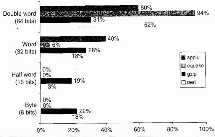
Figure A.29 Data reference size of four programs from SPEC2000. Although you can calculate an average size, it would be hard to claim the average is typical of programs.
