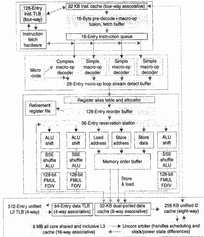
Figure 3.41 The Intel Core i7 pipeline structure shown with the memory system components. The total pipeline depth is 14 stages, with branch mispredictions costing 17 cycles. There are 48 load and 32 store buffers. The six independent functional units can each begin execution of a ready micro-op in the same cycle.
