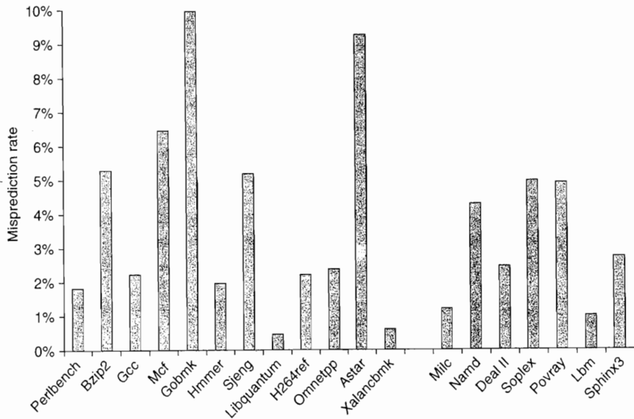
Figure 3.5 The misprediction rate for 19 of the SPECCPU2006 benchmarks versus the number of successfully retired branches is slightly higher on average for the integer benchmarks than for the FP (4% versus 3%). More importantly, it is much higher for a few benchmarks.
