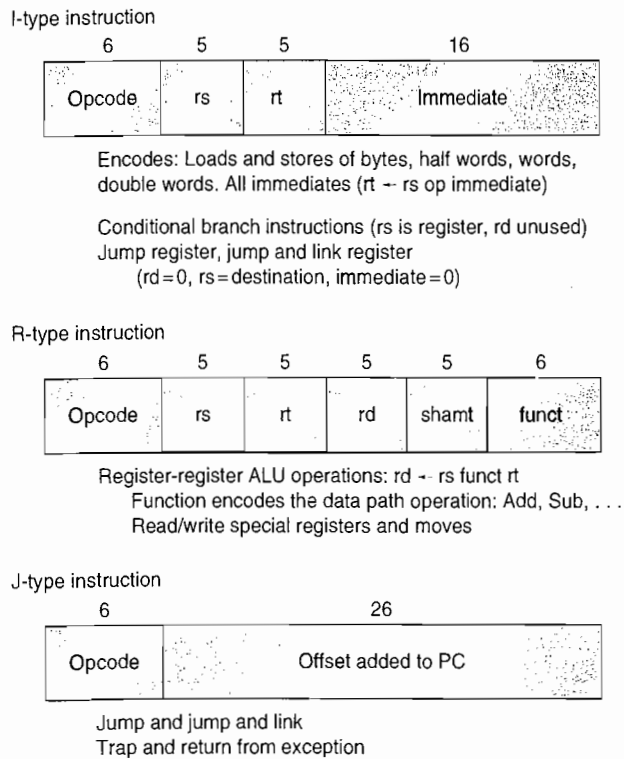
Figure A.22 Instruction layout for MIPS. All instructions are encoded in one of three types, with common fields in the same location in each format.
