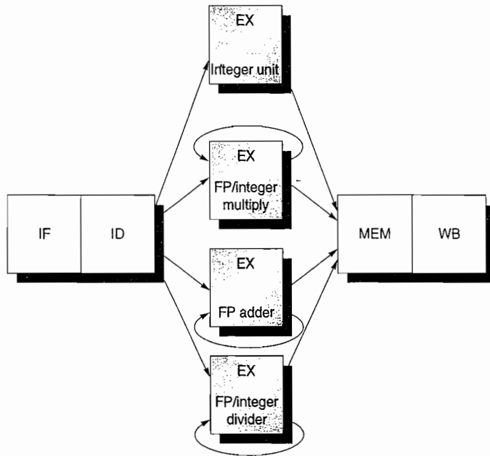
Figure C.33 The MIPS pipeline with three additional unpipelined, floating-point, functional units. Because only one instruction issues on every clock cycle, all instructions go through the standard pipeline for integer operations. The FP operations simply loop when they reach the EX stage. After they have finished the EX stage, they proceed to MEM and WB to complete execution.
