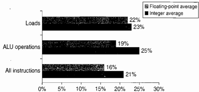
Figure A.9 About one-quarter of data transfers and ALU operations have an immediate operand. The bottom bars show that integer programs use immediates in about one-fifth of the instructions, while floating-point programs use immediates in about one-sixth of the instructions. For loads, the load immediate instruction loads 16 bits into either half of a 32-bit register. Load immediates are not loads in a strict sense because they do not access memory. Occasionally a pair of load immediates is used to load a 32-bit constant, but this is rare. (For ALU operations, shifts by a constant amount are included as operations with immediate operands.) The programs and computer used to collect these statistics are the same as in Figure A.8.
