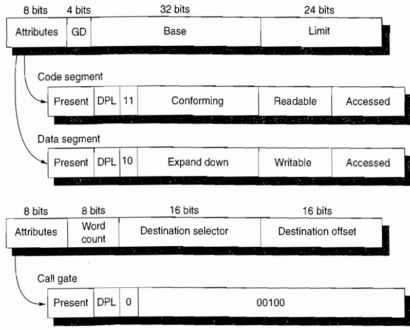
Figure B.26 The IA-32 segment descriptors are distinguished by bits in the attributes field. Base , limit , present , readable , and writable are all self-explanatory. D gives the default addressing size of the instructions: 16 bits or 32 bits. G gives the granularity of the segment limit: 0 means in bytes and 1 means in 4 KB pages. G is set to 1 when paging is turned on to set the size of the page tables. DPL means descriptor privilege level —this is checked against the code privilege level to see if the access will be allowed. Conforming says the code takes on the privilege level of the code being called rather than the privilege level of the caller; it is used for library routines. The expand-down field flips the check to let the base field be the high-water mark and the limit field be the low-water mark. As you might expect, this is used for stack segments that grow down. Word count controls the number of words copied from the current stack to the new stack on a call gate. The other two fields of the call gate descriptor, destination selector and destination offset , select the descriptor of the destination of the call and the offset into it, respectively. There are many more than these three segment descriptors in the IA-32 protection model.
