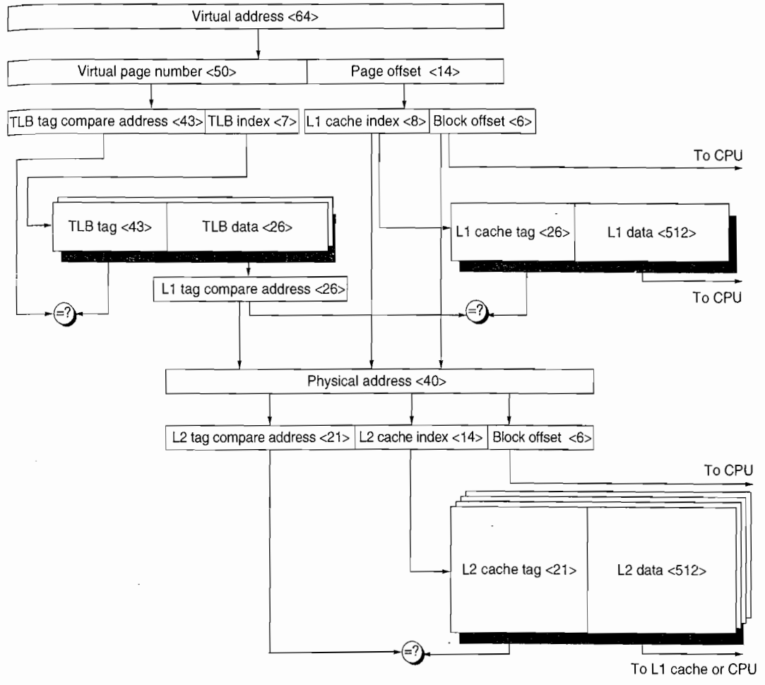
Figure B.17 The overall picture of a hypothetical memory hierarchy going from virtual address to L2 cache access. The page size is 16 KB. The TLB is two-way set associative with 256 entries. The L1 cache is a direct-mapped 16 KB, and the L2 cache is a four-way set associative with a total of 4 MB. Both use 64-byte blocks. The virtual address is 64 bits and the physical address is 40 bits.
