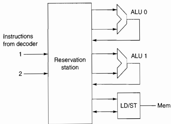
Figure 3.55 An out-of-order microarchitecture.
