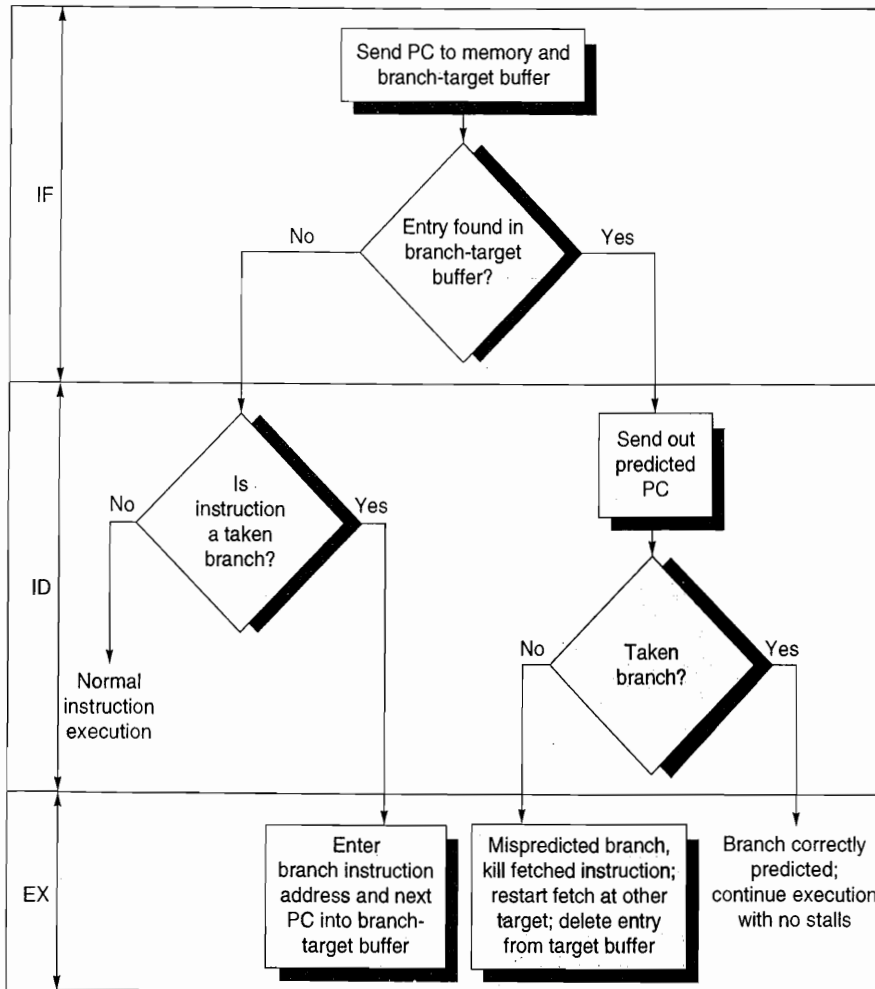
Figure 3.22 The steps involved in handling an instruction with a branch-target buffer.
