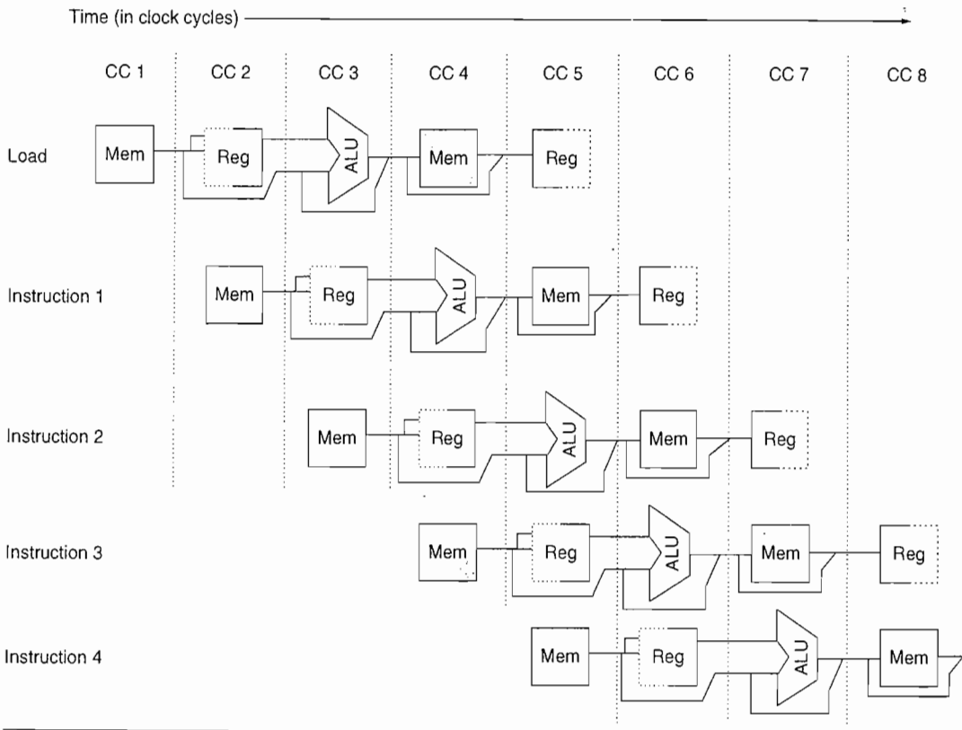
Figure C.4 A processor with only one memory port will generate a conflict whenever a memory reference occurs. In this example the load instruction uses the memory for a data access at the same time instruction 3 wants to fetch an instruction from memory.
