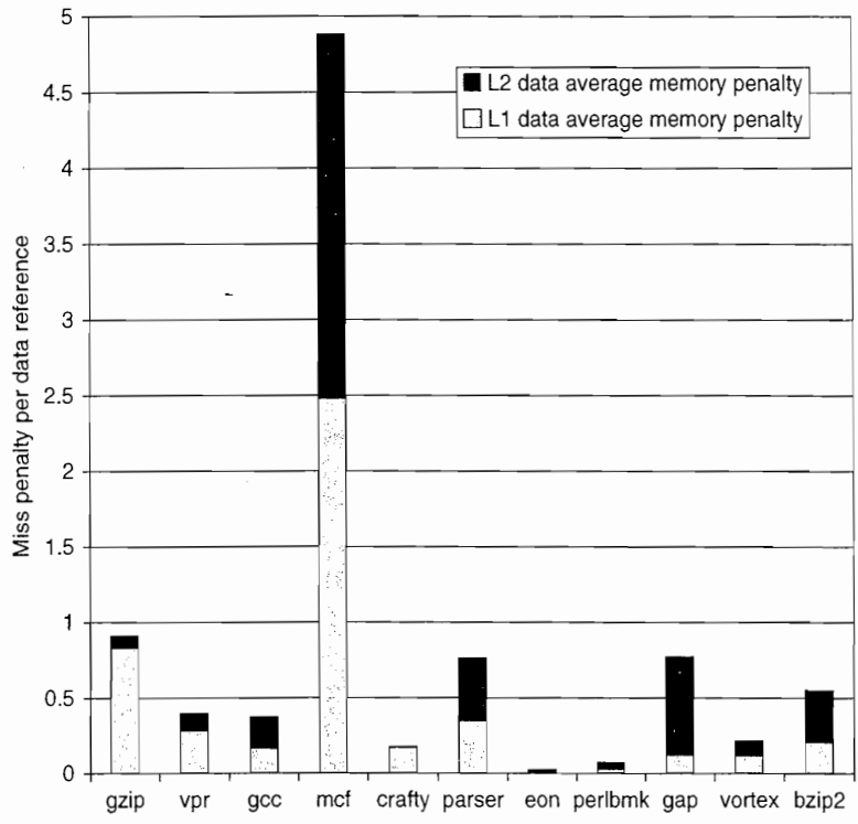
Figure 2.18 The average memory access penalty per data memory reference coming from L1 and L2 is shown for the ARM processor when running Minniespec. Although the miss rates for L1 are significantly higher, the L2 miss penalty, which is more than five times higher, means that the L2 misses can contribute significantly.
