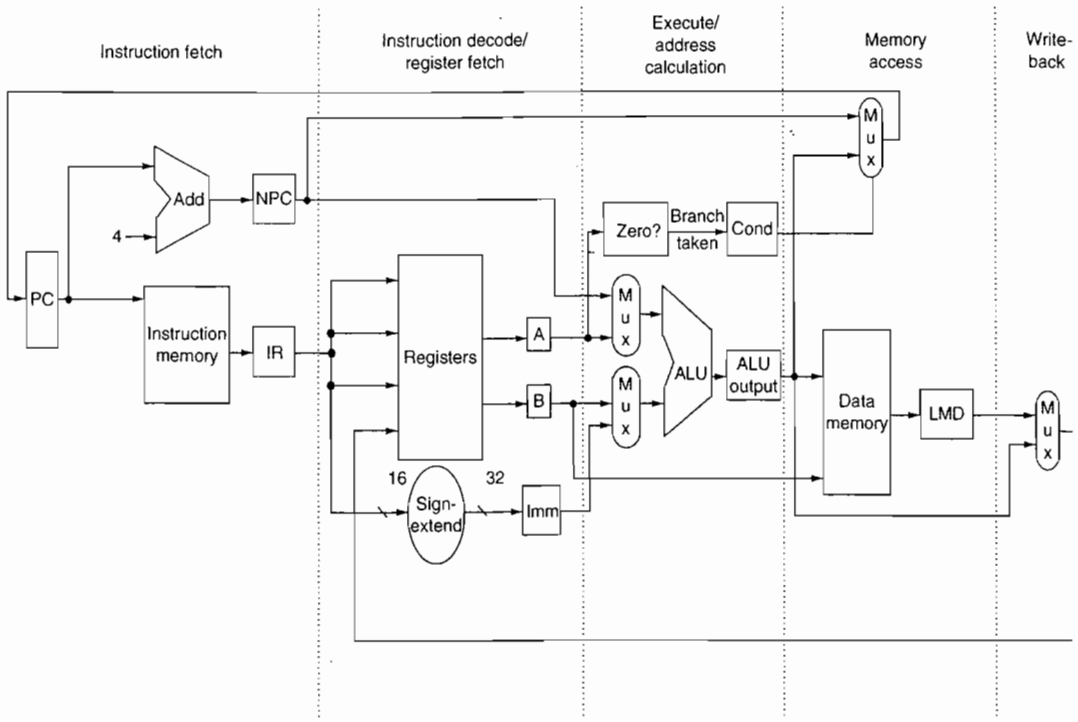
Figure C.21 The implementation of the MIPS data path allows every instruction to be executed in 4 or 5 clock cycles. Although the PC is shown in the portion of the data path that is used in instruction fetch and the registers are shown in the portion of the data path that is used in instruction decode/register fetch, both of these functional units are read as well as written by an instruction. Although we show these functional units in the cycle corresponding to where they are read, the PC is written during the memory access clock cycle and the registers are written during the write-back clock cycle. In both cases, the writes in later pipe stages are indicated by the multiplexer output (in memory access or write-back), which carries a value back to the PC or registers. These backward-flowing signals introduce much of the complexity of pipelining, since they indicate the possibility of hazards.
