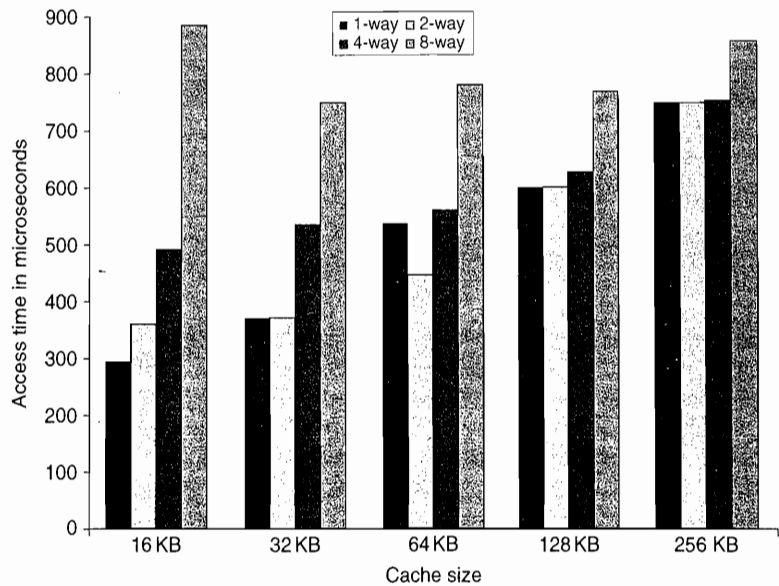
Figure 2.3 Access times generally increase as cache size and associativity are increased. These data come from the CACTI model 6.5 by Tarjan, Thoziyoor, and Jouppi [2005]. The data assume a 40 nm feature size (which is between the technology used in Intel's fastest and second fastest versions of the i7 and the same as the technology used in the fastest ARM embedded processors), a single bank, and 64-byte blocks. The assumptions about cache layout and the complex trade-offs between interconnect delays (that depend on the size of a cache block being accessed) and the cost of tag checks and multiplexing lead to results that are occasionally surprising, such as the lower access time for a 64 KB with two-way set associativity versus direct mapping. Similarly, the results with eight-way set associativity generate unusual behavior as cache size is increased. Since such observations are highly dependent on technology and detailed design assumptions, tools such as CACTI serve to reduce the search space rather than precision analysis of the trade-offs.
