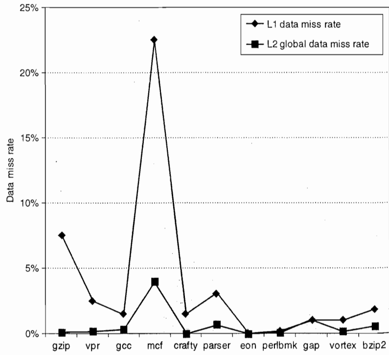
Figure 2.17 The data miss rate for ARM with a 32 KB L1 and the global data miss rate for a 1 MB L2 using the integer Minnespec benchmarks are significantly affected by the applications. Applications with larger memory footprints tend to have higher miss rates in both L1 and L2. Note that the L2 rate is the global miss rate, that is counting all references, including those that hit in L1. Mcf is known as a cache buster.
