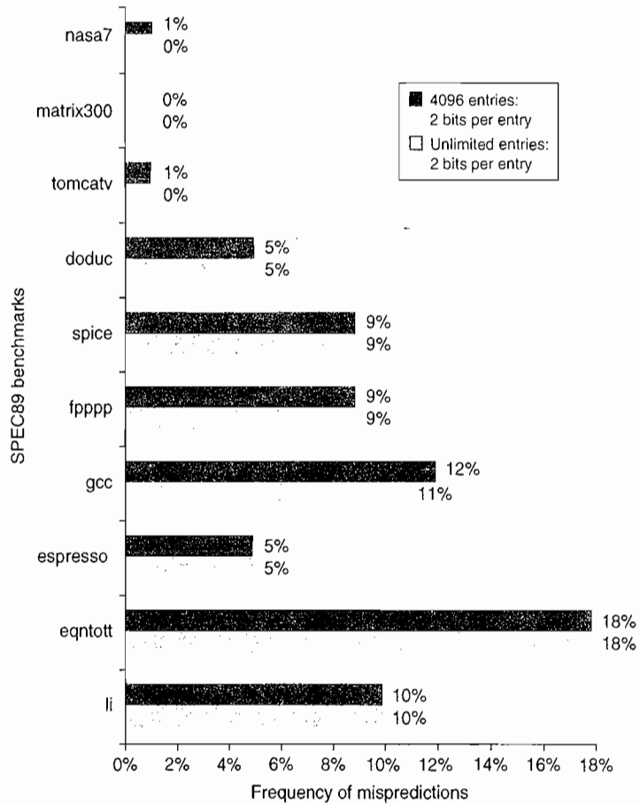
Figure C.20 Prediction accuracy of a 4096-entry 2-bit prediction buffer versus an infinite buffer for the SPEC89 benchmarks. Although these data are for an older version of a subset of the SPEC benchmarks, the results would be comparable for newer versions with perhaps as many as 8K entries needed to match an infinite 2-bit predictor.
