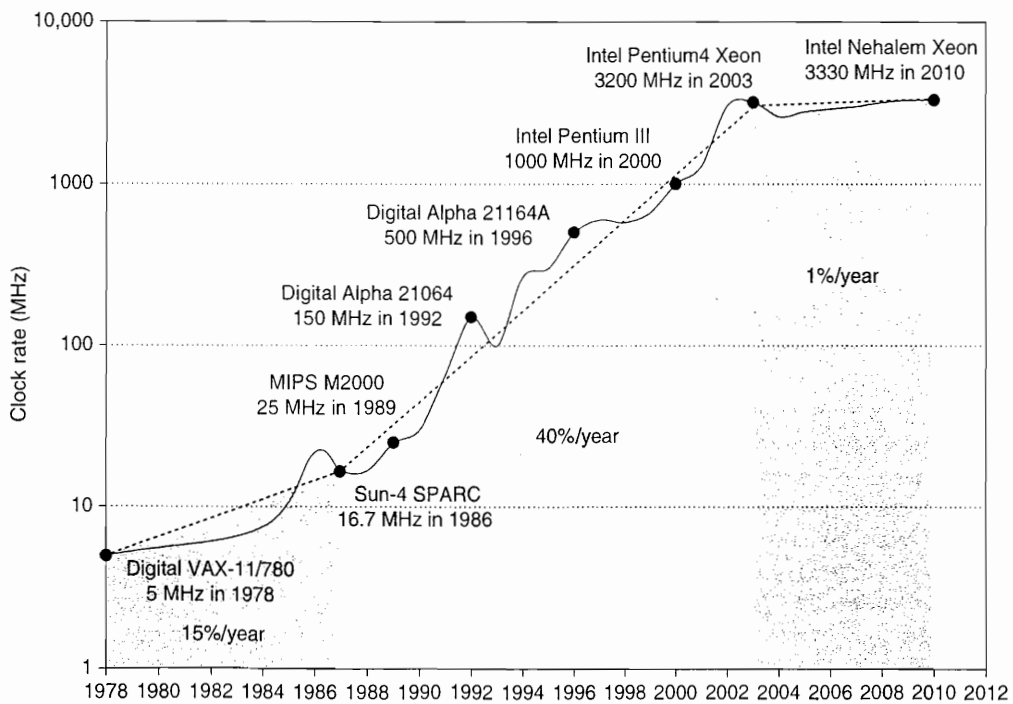
Figure 1.11 Growth in clock rate of microprocessors in Figure 1.1. Between 1978 and 1986, the clock rate improved less than 15% per year while performance improved by 25% per year. During the “renaissance period” of 52% performance improvement per year between 1986 and 2003, clock rates shot up almost 40% per year. Since then, the clock rate has been nearly flat, growing at less than 1% per year, while single processor performance improved at less than 22% per year.
