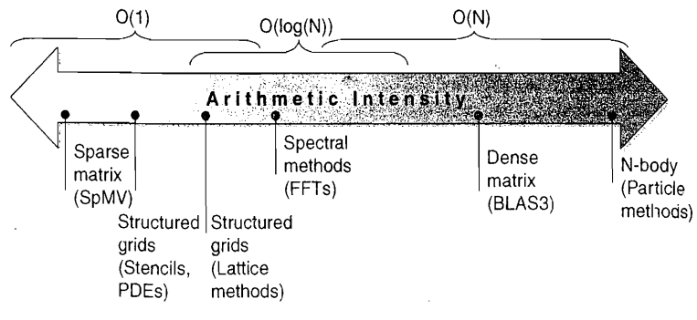
Figure 4.10 Arithmetic intensity, specified as the number of floating-point operations to run the program divided by the number of bytes accessed in main memory [Williams et al. 2009]. Some kernels have an arithmetic intensity that scales with problem size, such as dense matrix, but there are many kernels with arithmetic intensities independent of problem size.
