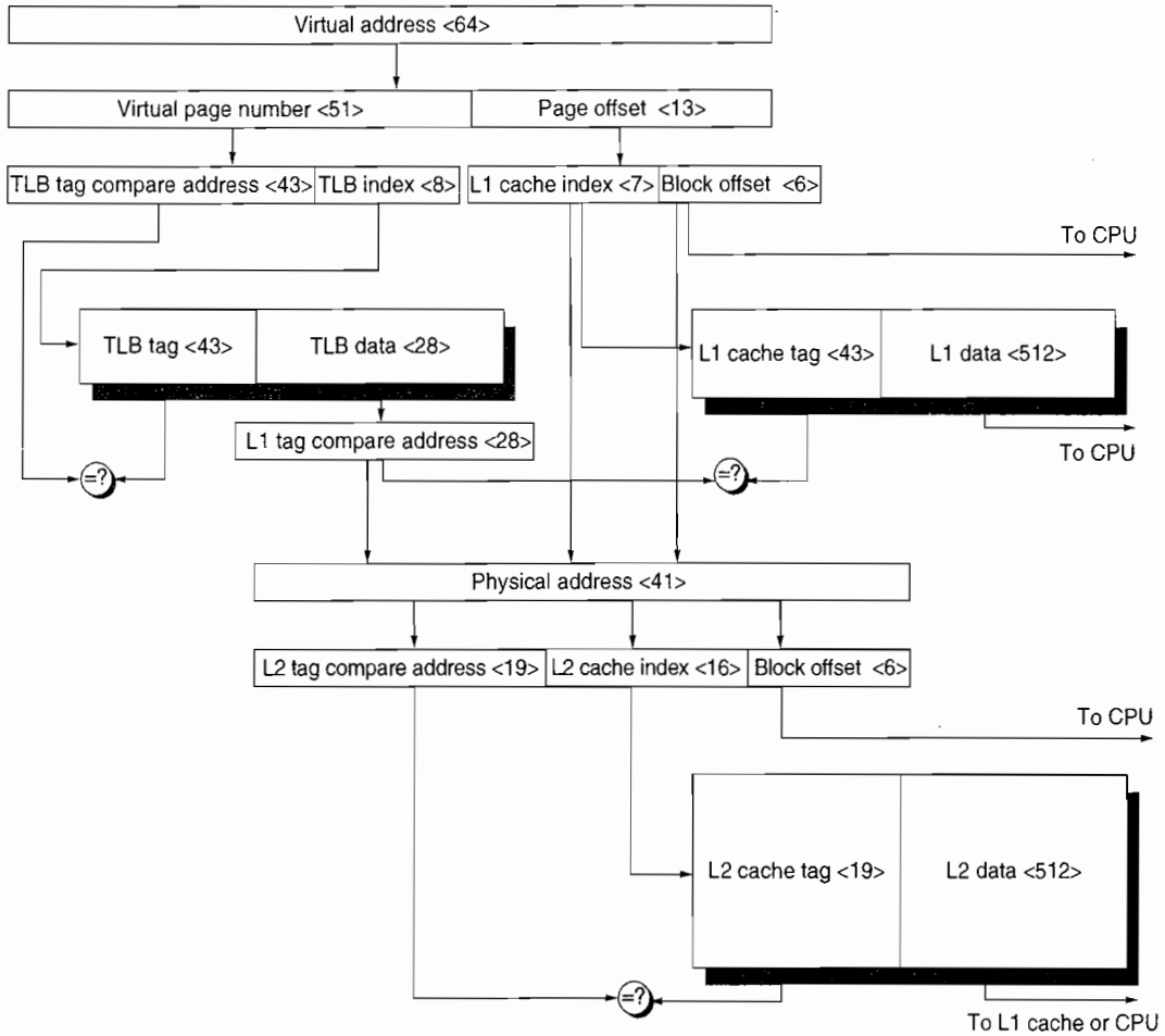
Figure B.25 The overall picture of a hypothetical memory hierarchy going from virtual address to L2 cache access. The page size is 8 KB. The TLB is direct mapped with 256 entries. The L1 cache is a direct-mapped 8 KB, and the L2 cache is a direct-mapped 4 MB. Both use 64-byte blocks. The virtual address is 64 bits and the physical address is 41 bits. The primary difference between this simple figure and a real cache is replication of pieces of this figure.
