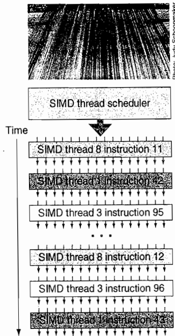
Figure 4.16 Scheduling of threads of SIMD instructions. The scheduler selects a ready thread of SIMD instructions and issues an instruction synchronously to all the SIMD Lanes executing the SIMD thread. Because threads of SIMD instructions are independent, the scheduler may select a different SIMD thread each time.
