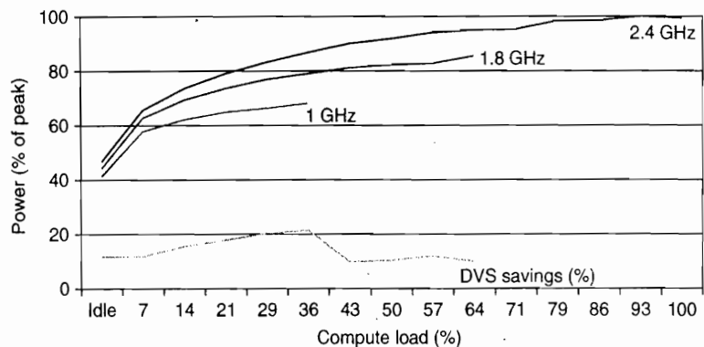
Figure 1.12 Energy savings for a server using an AMD Opteron microprocessor, 8 GB of DRAM, and one ATA disk. At 1.8 GHz, the server can only handle up to two-thirds of the workload without causing service level violations, and, at 1.0 GHz, it can only safely handle one-third of the workload. (Figure 5.11 in Barroso and Hölzle [2009].)
