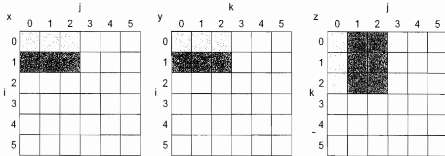
Figure 2.9 The age of accesses to the arrays x , y , and z when B = 3 . Note that, in contrast to Figure 2.8, a smaller number of elements is accessed.
