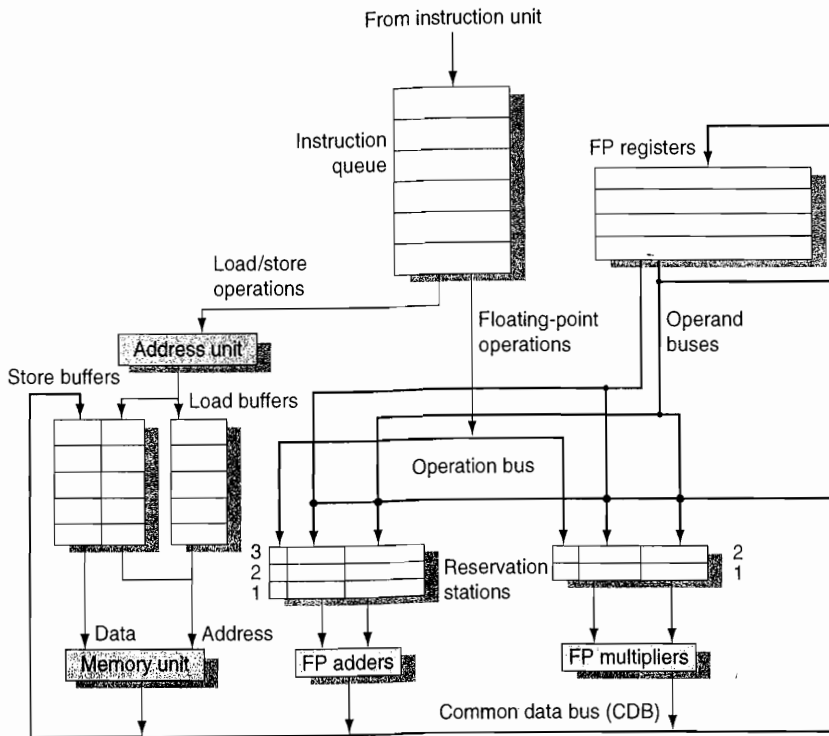
Figure 3.6 The basic structure of a MIPS floating-point unit using Tomasulo's algorithm. Instructions are sent from the instruction unit into the instruction queue from which they are issued in first-in, first-out (FIFO) order. The reservation stations include the operation and the actual operands, as well as information used for detecting and resolving hazards. Load buffers have three functions: (1) hold the components of the effective address until it is computed, (2) track outstanding loads that are waiting on the memory, and (3) hold the results of completed loads that are waiting for the CDB. Similarly, store buffers have three functions: (1) hold the components of the effective address until it is computed, (2) hold the destination memory addresses of outstanding stores that are waiting for the data value to store, and (3) hold the address and value to store until the memory unit is available. All results from either the FP units or the load unit are put on the CDB, which goes to the FP register file as well as to the reservation stations and store buffers. The FP adders implement addition and subtraction, and the FP multipliers do multiplication and division.
