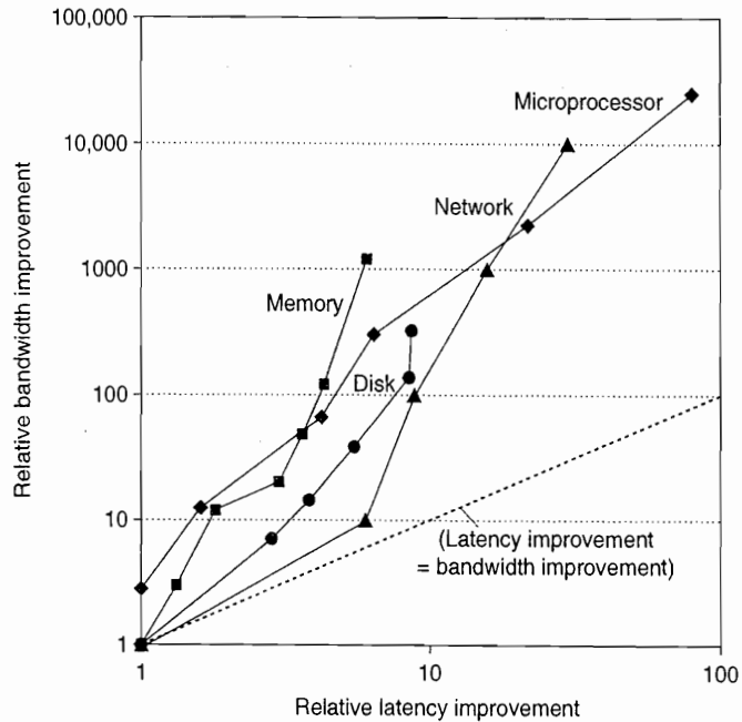
Figure 1.9 Log-log plot of bandwidth and latency milestones from Figure 1.10 relative to the first milestone. Note that latency improved 6X to 80X while bandwidth improved about 300X to 25,000X. Updated from Patterson [2004].
