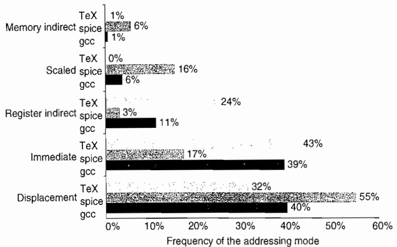
Figure A.7 Summary of use of memory addressing modes (including immediates). These major addressing modes account for all but a few percent (0% to 3%) of the memory accesses. Register modes, which are not counted, account for one-half of the operand references, while memory addressing modes (including immediate) account for the other half. Of course, the compiler affects what addressing modes are used; see Section A.8. The memory indirect mode on the VAX can use displacement, autoincrement, or autodecrement to form the initial memory address; in these programs, almost all the memory indirect references use displacement mode as the base. Displacement mode includes all displacement lengths (8, 16, and 32 bits). The PC-relative addressing modes, used almost exclusively for branches, are not included. Only the addressing modes with an average frequency of over 1% are shown.
