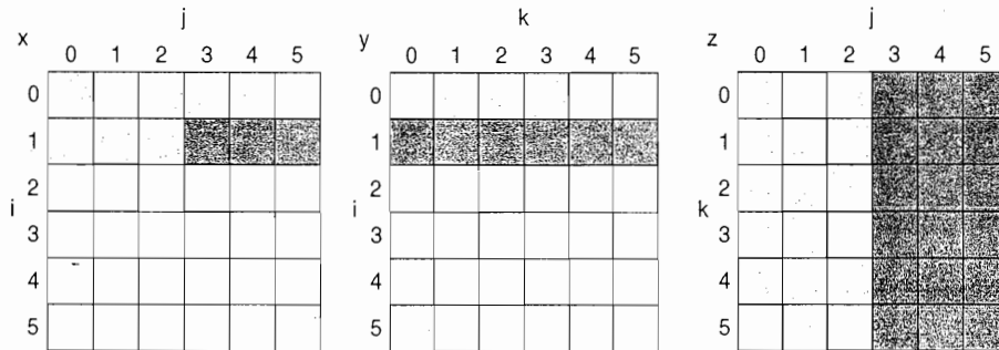
Figure 2.8 A snapshot of the three arrays x , y , and z when N = 6 and i = 1 . The age of accesses to the array elements is indicated by shade: white means not yet touched, light means older accesses, and dark means newer accesses. Compared to Figure 2.9, elements of y and z are read repeatedly to calculate new elements of x . The variables i , j , and k are shown along the rows or columns used to access the arrays.
