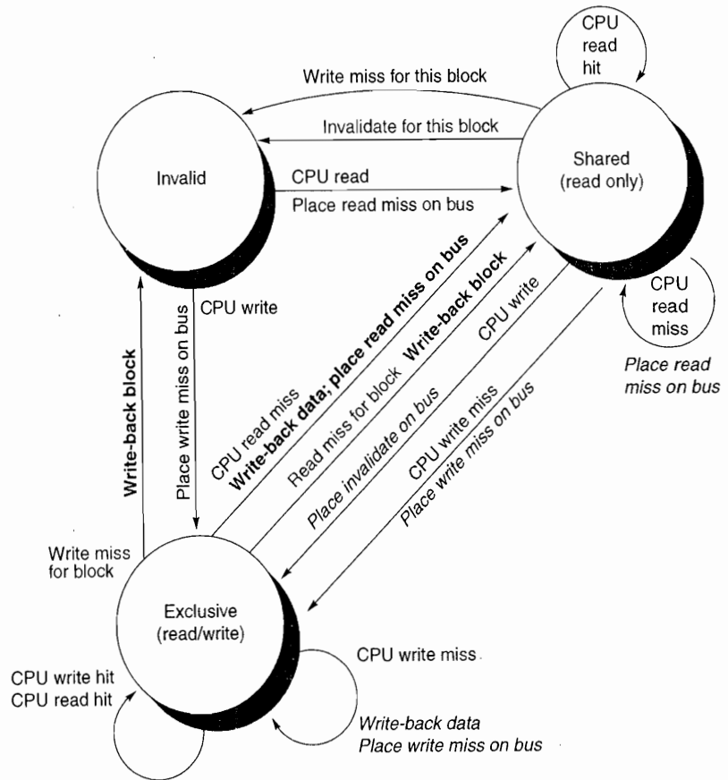
Figure 5.7 Cache coherence state diagram with the state transitions induced by the local processor shown in black and by the bus activities shown in gray. As in Figure 5.6, the activities on a transition are shown in bold.
