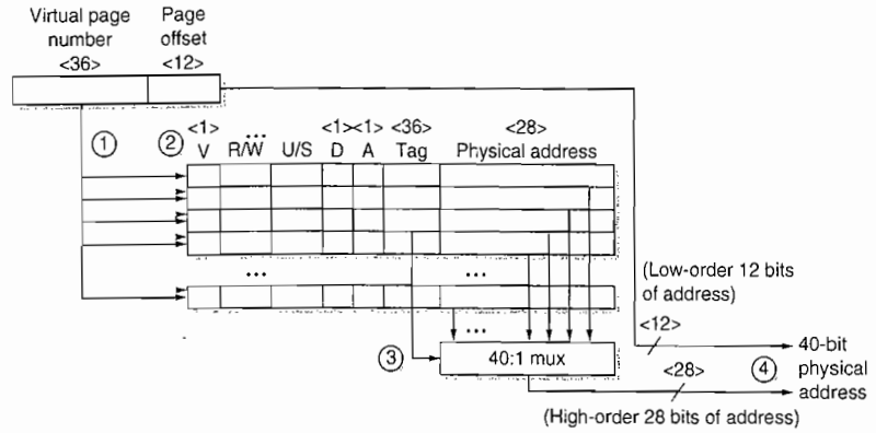
Figure B.24 Operation of the Oporteron data TLB during address translation. The four steps of a TLB hit are shown as circled numbers. This TLB has 40 entries. Section B.5 describes the various protection and access fields of an Oporteron page table entry.
