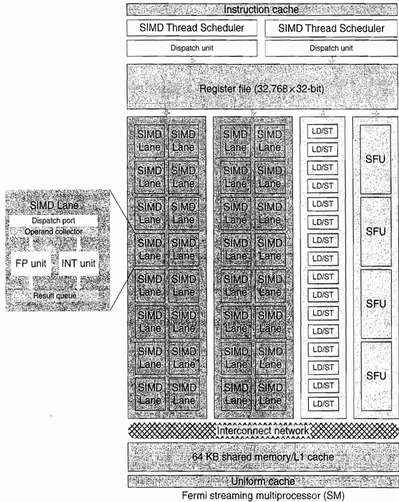
Figure 4.20 Block diagram of the multithreaded SIMD Processor of a Fermi GPU. Each SIMD Lane has a pipelined floating-point unit, a pipelined integer unit, some logic for dispatching instructions and operands to these units, and a queue for holding results. The four Special Function units (SFUs) calculate functions such as square roots, reciprocals, sines, and cosines.
