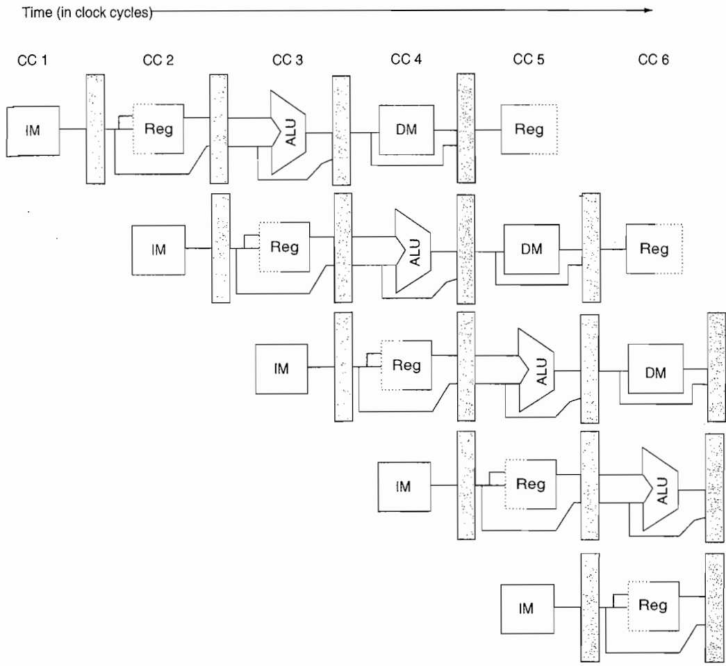
Figure C.3 A pipeline showing the pipeline registers between successive pipeline stages. Notice that the registers prevent interference between two different instructions in adjacent stages in the pipeline. The registers also play the critical role of carrying data for a given instruction from one stage to the other. The edge-triggered property of registers—that is, that the values change instantaneously on a clock edge—is critical. Otherwise, the data from one instruction could interfere with the execution of another!
