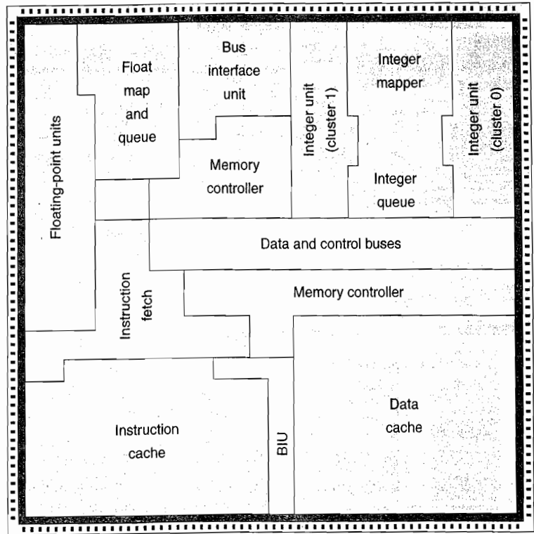
Figure 2.33 Floorplan of the Alpha 21264 [Kessler 1999].
