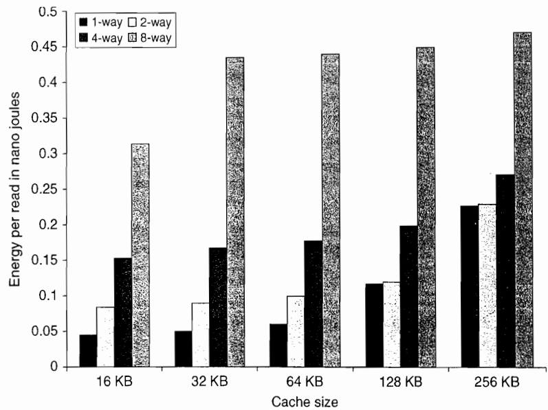
Figure 2.4 Energy consumption per read increases as cache size and associativity are increased. As in the previous figure, CACTI is used for the modeling with the same technology parameters. The large penalty for eight-way set associative caches is due to the cost of reading out eight tags and the corresponding data in parallel.
