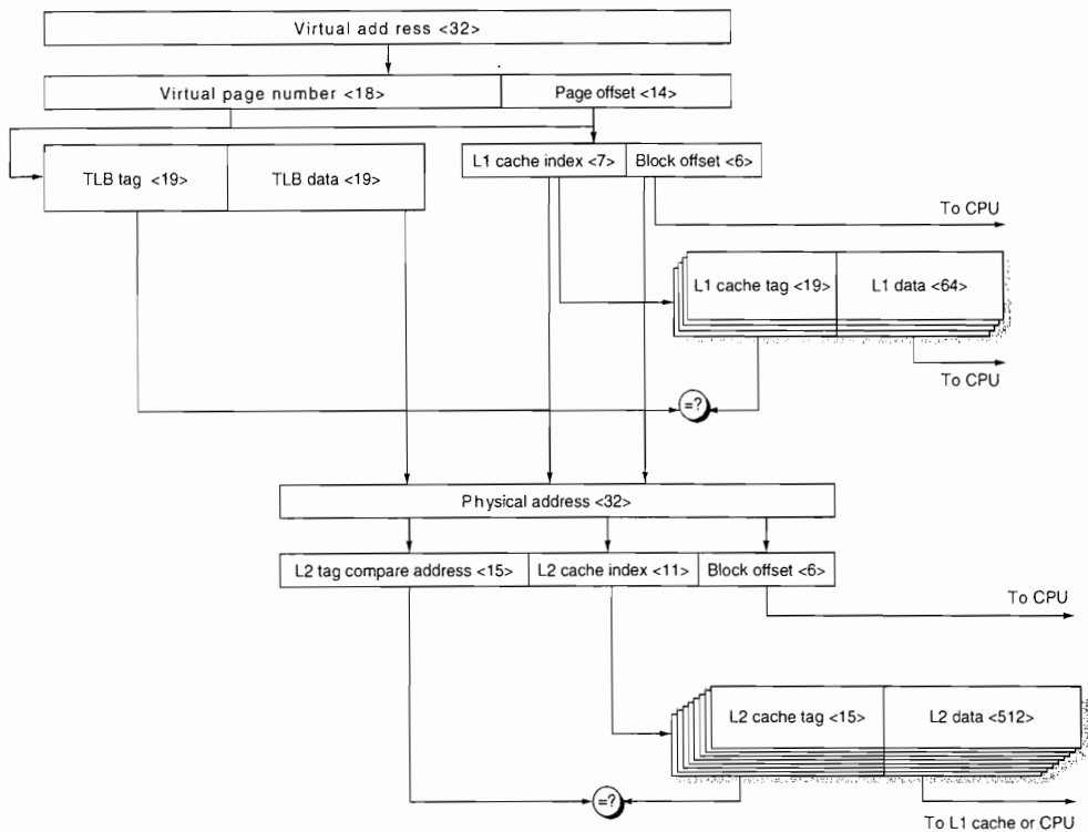
Figure 2.16 The virtual address, physical address, indexes, tags, and data blocks for the ARM Cortex-A8 data caches and data TLB. Since the instruction and data hierarchies are symmetric, we show only one. The TLB (instruction or data) is fully associative with 32 entries. The L1 cache is four-way set associative with 64-byte blocks and 32 KB capacity. The L2 cache is eight-way set associative with 64-byte blocks and 1 MB capacity. This figure doesn't show the valid bits and protection bits for the caches and TLB, nor the use of the way prediction bits that would dictate the predicted bank of the L1 cache.
