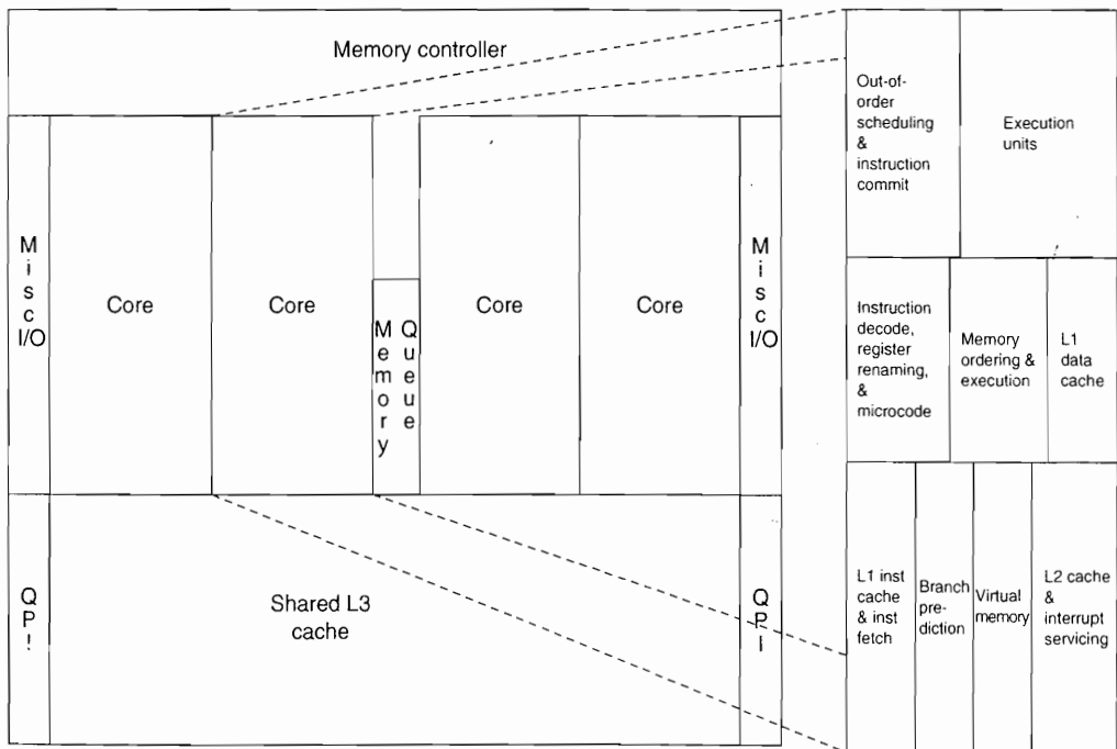
Figure 1.14 Floorplan of Core i7 die in Figure 1.13 on left with close-up of floorplan of second core on right.
