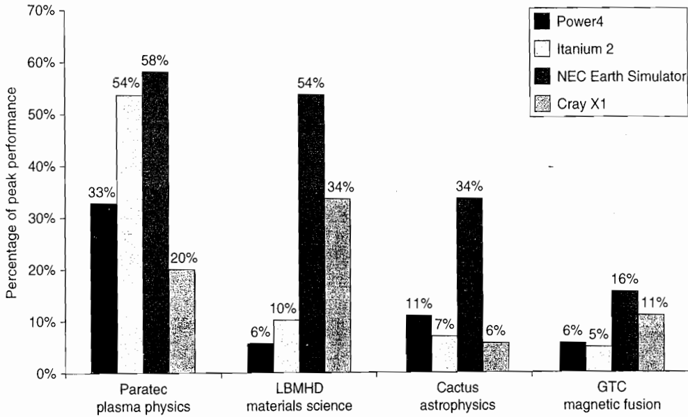
Figure 1.20 Percentage of peak performance for four programs on four multiprocessors scaled to 64 processors. The Earth Simulator and X1 are vector processors (see Chapter 4 and Appendix G). Not only did they deliver a higher fraction of peak performance, but they also had the highest peak performance and the lowest clock rates. Except for the Paratec program, the Power 4 and Itanium 2 systems delivered between 5% and 10% of their peak. From Oliner et al. [2004].
