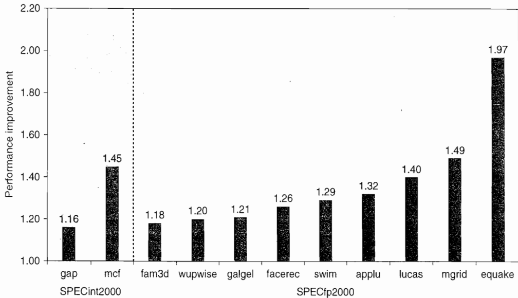
Figure 2.10 Speedup due to hardware prefetching on Intel Pentium 4 with hardware prefetching turned on for 2 of 12 SPECint2000 benchmarks and 9 of 14 SPECfp2000 benchmarks. Only the programs that benefit the most from prefetching are shown; prefetching speeds up the missing 15 SPEC benchmarks by less than 15% [Singhal 2004].
