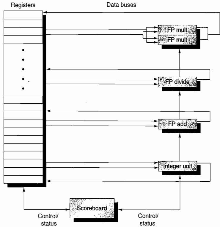
Figure C.54 The basic structure of a MIPS processor with a scoreboard. The scoreboard's function is to control instruction execution (vertical control lines). All of the data flow between the register file and the functional units over the buses (the horizontal lines, called trunks in the CDC 6600). There are two FP multipliers, an FP divider, an FP adder, and an integer unit. One set of buses (two inputs and one output) serves a group of functional units. The details of the scoreboard are shown in Figures C.55 to C.58.
