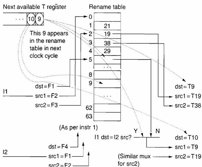
Figure 3.52 Rename table and on-the-fly register substitution logic for superscalar machines. (Note that src is source, and dest is destination.)
