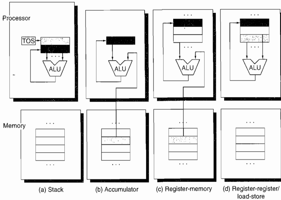
Figure A.1 Operand locations for four instruction set architecture classes. The arrows indicate whether the operand is an input or the result of the arithmetic-logical unit (ALU) operation, or both an input and result. Lighter shades indicate inputs, and the dark shade indicates the result. In (a), a Top Of Stack register (TOS) points to the top input operand, which is combined with the operand below. The first operand is removed from the stack, the result takes the place of the second operand, and TOS is updated to point to the result. All operands are implicit. In (b), the Accumulator is both an implicit input operand and a result. In (c), one input operand is a register, one is in memory, and the result goes to a register. All operands are registers in (d) and, like the stack architecture, can be transferred to memory only via separate instructions: push or pop for (a) and load or store for (d).
