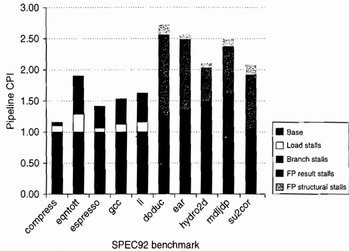
Figure C.52 The pipeline CPI for 10 of the SPEC92 benchmarks, assuming a perfect cache. The pipeline CPI varies from 1.2 to 2.8. The leftmost five programs are integer programs, and branch delays are the major CPI contributor for these. The rightmost five programs are FP, and FP result stalls are the major contributor for these. Figure C.53 shows the numbers used to construct this plot.
