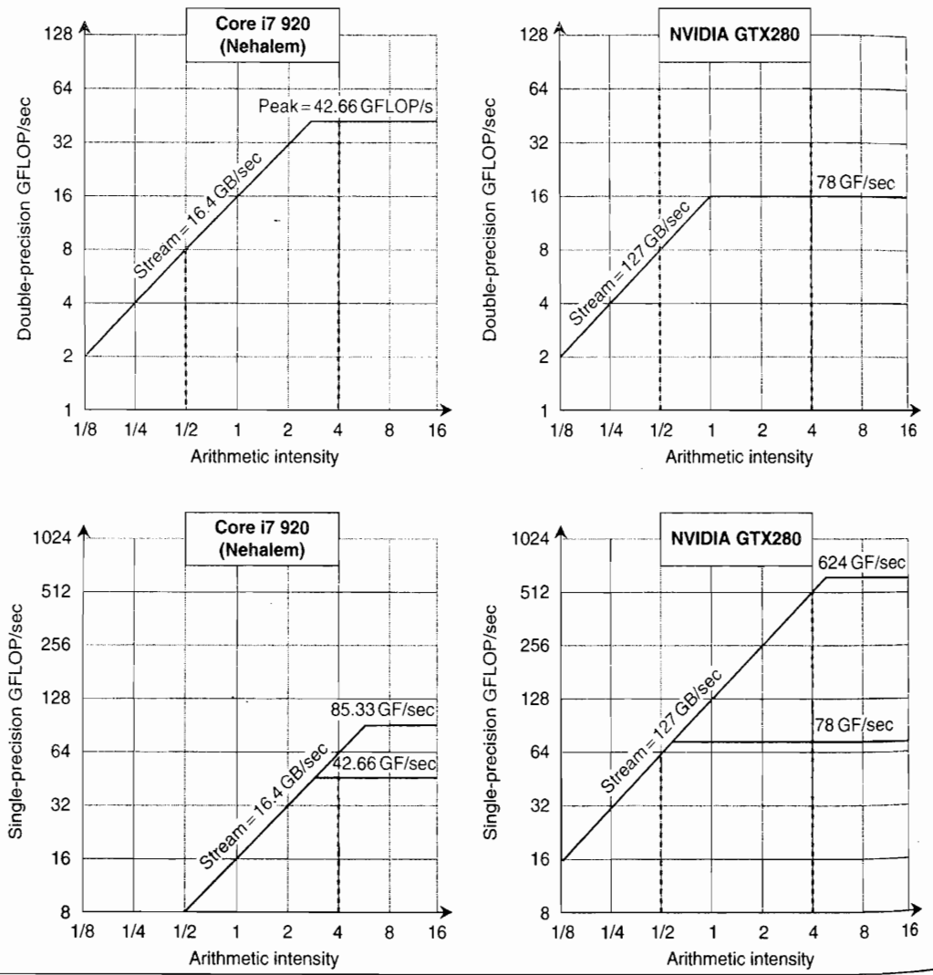
Figure 4.28 Roofline model [Williams et al. 2009]. These rooflines show double-precision floating-point performance in the top row and single-precision performance in the bottom row. (The DP FP performance ceiling is also in the bottom row to give perspective.) The Core i7 920 on the left has a peak DP FP performance of 42.66 GFLOP/sec, a SP FP peak of 85.33 GFLOP/sec, and a peak memory bandwidth of 16.4 GBytes/sec. The NVIDIA GTX 280 has a DP FP peak of 78 GFLOP/sec, SP FP peak of 624 GFLOP/sec, and 127 GBytes/sec of memory bandwidth. The dashed vertical line on the left represents an arithmetic intensity of 0.5 FLOP/byte. It is limited by memory bandwidth to no more than 8 DP GFLOP/sec or 8 SP GFLOP/sec on the Core i7. The dashed vertical line to the right has an arithmetic intensity of 4 FLOP/byte. It is limited only computationally to 42.66 DP GFLOP/sec and 64 SP GFLOP/sec on the Core i7 and 78 DP GFLOP/sec and 512 DP GFLOP/sec on the GTX 280. To hit the highest computation rate on the Core i7 you need to use all 4 cores and SSE instructions with an equal number of multiplies and adds. For the GTX 280, you need to use fused multiply-add instructions on all multithreaded SIMD processors. Guz et al. [2009] have an interesting analytic model for these two architectures.
