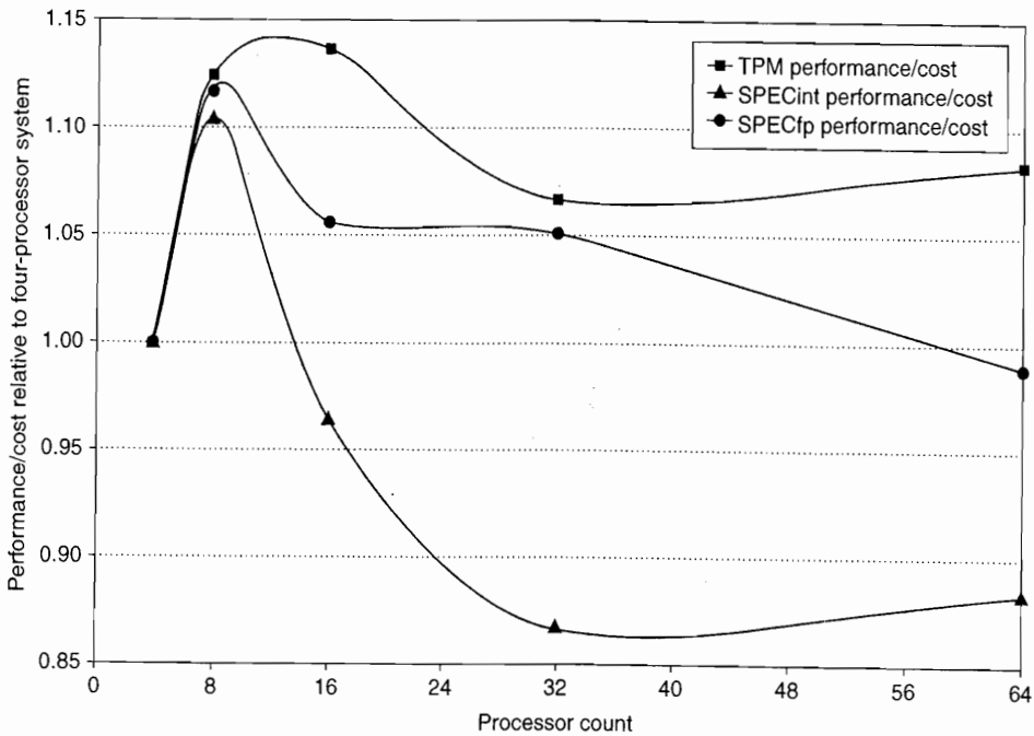
Figure 5.33 The performance/cost relative to a 4-processor system for three benchmarks run on an IBM eServer p5 multiprocessor containing from 4 to 64 processors shows that the larger processor counts can be as cost effective as the 4-processor configuration. For TPC-C the configurations are those used in the official runs, which means that disk and memory scale nearly linearly with processor count, and a 64-processor machine is approximately twice as expensive as a 32-processor version. In contrast, the disk and memory are scaled more slowly (although still faster than necessary to achieve the best SPECrate at 64 processors). In particular, the disk configurations go from one drive for the 4-processor version to four drives (140 GB) for the 64-processor version. Memory is scaled from 8 GB for the 4-processor system to 20 GB for the 64-processor system.
