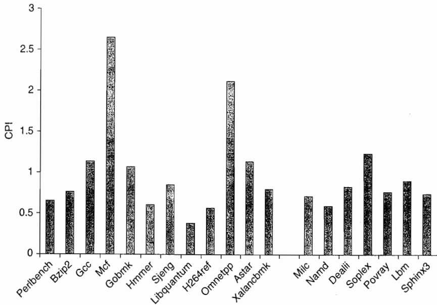
Figure 3.43 The CPI for the 19 SPEC CPU2006 benchmarks shows an average CPI for 0.83 for both the FP and integer benchmarks, although the behavior is quite different. In the integer case, the CPI values range from 0.44 to 2.66 with a standard deviation of 0.77, while the variation in the FP case is from 0.62 to 1.38 with a standard deviation of 0.25. The data in this section were collected by Professor Lu Peng and Ph.D. student Ying Zhang, both of Louisiana State University.
